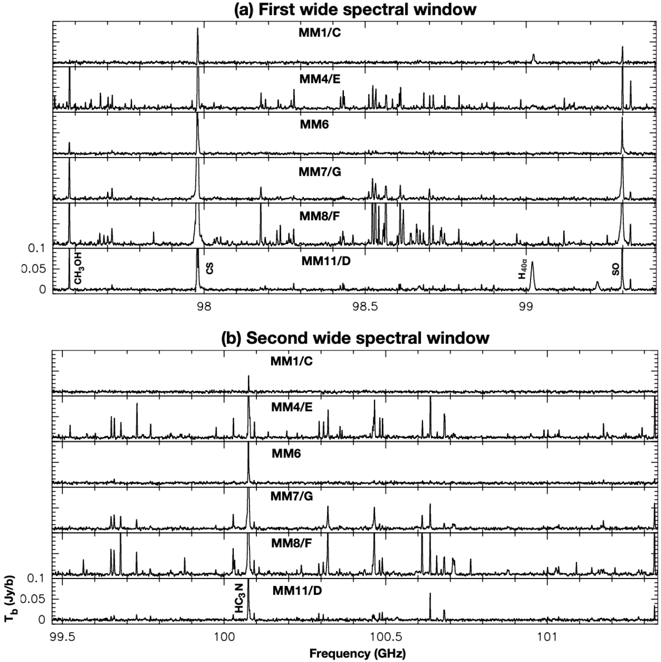
Figure 13. The line spectra of the two wide spectral window averaged over 2'' at each core of G9.62+0.19.
