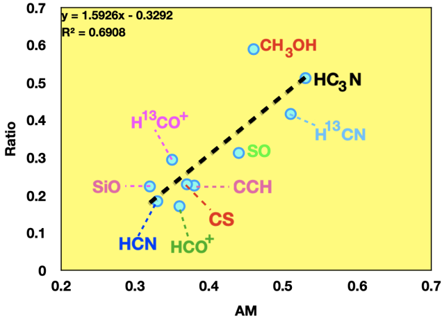
Figure 19. The ratio of S_V^{12m} to S_V^{ACA} is plotted as a function of the alignment measurement ( AM ) in HOG analysis for 3 mm continuum and molecular line emission.
