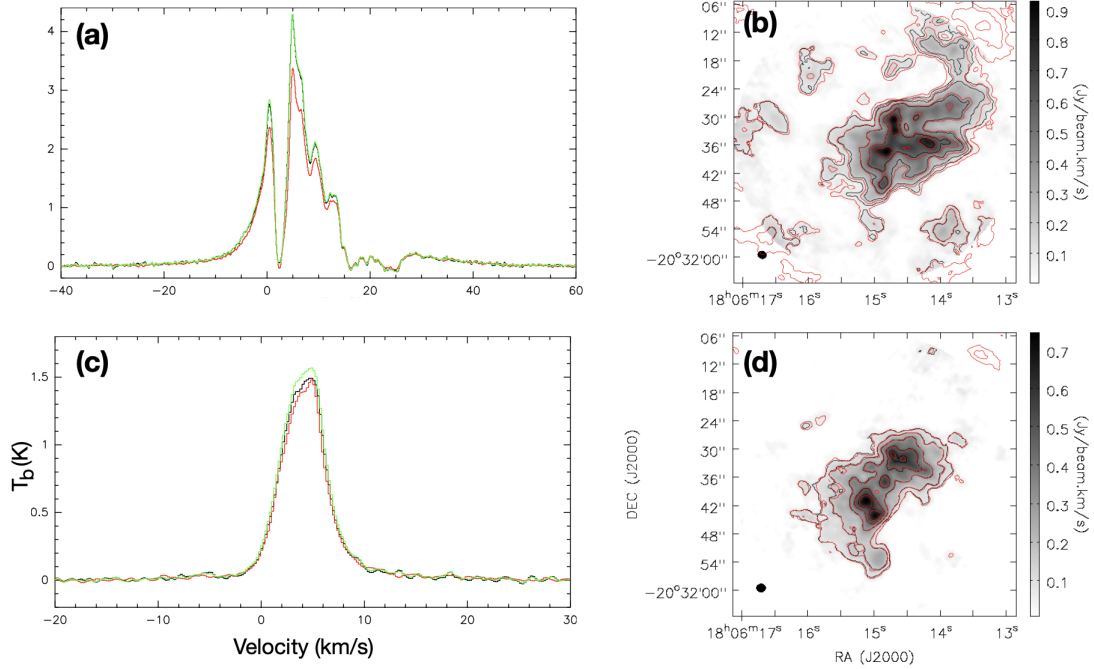
Figure 4. (a) \text{HCO}^+ spectra in G9.62+0.19 averaged over a 30'' region at the central position (R.A.(J2000)=18:06:14.99, decl.(J2000)=-20:31:35.4). The spectra from ACA data, 12-m array data and combined 12-m and ACA data are shown in black, red and green, respectively. (b) Comparison of the integrated intensity maps of \text{HCO}^+ emission from 12-m array data (gray image and black contours) and combined data (red contours). The contours are [0.1, 0.2, 0.4, 0.6, 0.8] \times F_{\text{peak}} . The peak integrated intensities ( F_{\text{peak}} ) in 12-m array data and in combined data are 0.93 and 0.96 \text{Jy beam}^{-1} \text{km s}^{-1} , respectively. (c) Same as in panel a but for \text{H}^{13}\text{CO}^+ . (d) Same as in panel b but for \text{H}^{13}\text{CO}^+ . The peak integrated intensities ( F_{\text{peak}} ) in 12-m array data and in combined data are the same as 0.75 \text{Jy beam}^{-1} \text{km s}^{-1} .
