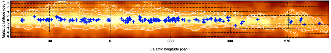
Figure 1. Galactic distribution of the ATOMS targets (""). The background image and contours show Planck 857 GHz emission. The contours are from 34.6 to 874.5 MJy/sr with 10 steps on a logarithmic scale.
