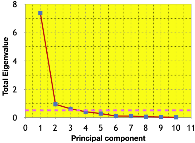
Figure 14. The eigenvalue against the component number of the 10 principal components (PCs). The dashed line marks an eigenvalue threshold of 0.5.
