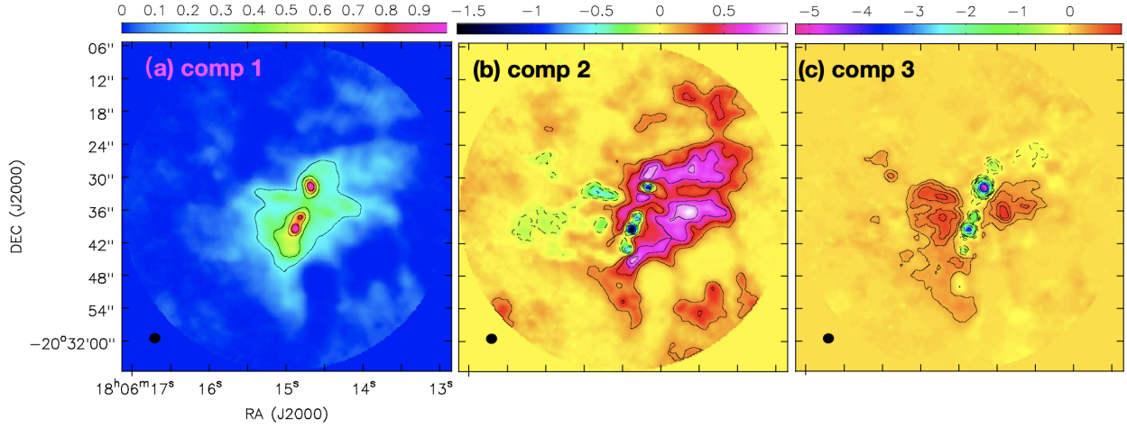
Figure 15. Constructed images of the first three PCs. The images are normalized to their maximum values. (a) Principal Component 1. The contours are 0.2,0.4,0.6,0.8 (b) Principal Component 2. The contours are -1.5,-1.3,-1.1,-0.1,0.2,0.4,0.6,0.8 (c) Principal Component 3. The contours are -5,-4,-3,-2,-1,-0.8,-0.6,-0.4,-0.2,0.2,0.4,0.6,0.8.
