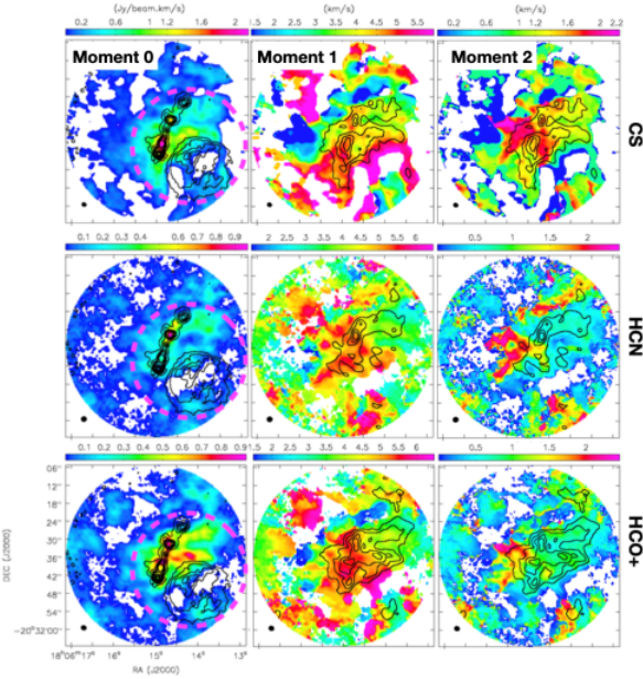
Figure A1. The left, middle and right columns present the integrated intensity (Moment 0) maps, intensity-weighted velocity maps (Moment 1) and intensity-weighted velocity dispersion (Moment 2) maps of G9.62+0.19 for the gas tracers indicated on the right of each row. The names of tracers are labeled to the right. The contours on Moment 0 maps show the 3 mm continuum emission. The contour levels are [0.01, 0.03, 0.05, 0.07, 0.1, 0.2, 0.4, 0.6, 0.8] \times 74.1 \text{ mJy beam}^{-1} . The contours on Moment 1 and Moment 2 maps show the corresponding integrated intensity maps of various gas tracers. The contours are [0.2, 0.4, 0.6, 0.8] \times F_{\text{peak}} . The peak integrated intensities ( F_{\text{peak}} ) for CS, HCN, HCO + are 2.16, 0.97, and 0.93 \text{Jy beam}^{-1} \text{ km s}^{-1} , respectively. The magenta dashed circle on Moment 0 map shows the clump boundary traced by H 13 CN.
