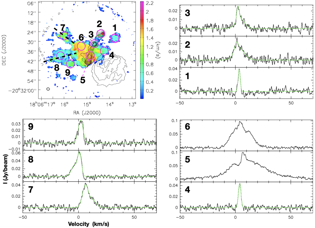
Figure 10. SiO spectra averaged over 5'' regions at nine positions across G9.62+0.19. The upper left panel shows the Moment 2 map of SiO overlaid on 3 mm continuum emission contours. The contour levels are the same as in Figure 5. The magenta circles mark the positions where the SiO spectra are extracted. The two black dashed lines mark the elongated structures that may be related to colliding flows. The other panels show the averaged SiO spectra at each position. The green lines are gaussian fits.
