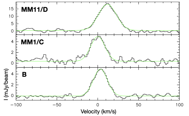
Figure 6. Source-averaged H 40α RRL in G9.62+0.19. The green lines are gaussian fits.
