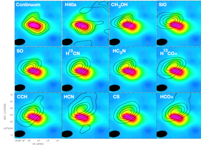
Figure 7. The integrated intensity maps from the ACA images of molecular line emission in G9.62+0.19 are shown in contours. The background color image is the 3 mm continuum emission. The contour levels are [0.2, 0.4, 0.6, 0.8] \times F_{\text{peak}} . The F_{\text{peak}} for various tracers are: Continuum: 0.225 \text{ Jy beam}^{-1} ; \text{H}_{40\alpha} : 7.8 \text{ Jy beam}^{-1} \text{ km s}^{-1} ; \text{CH}_3\text{OH} : 10.3 \text{ Jy beam}^{-1} \text{ km s}^{-1} ; \text{SiO} : 10.3 \text{ Jy beam}^{-1} \text{ km s}^{-1} ; \text{SO} : 28.8 \text{ Jy beam}^{-1} \text{ km s}^{-1} ; \text{H}^{13}\text{CN} : 15.3 \text{ Jy beam}^{-1} \text{ km s}^{-1} ; \text{HC}_3\text{N} : 34.5 \text{ Jy beam}^{-1} \text{ km s}^{-1} ; \text{H}^{13}\text{CO}^+ : 15.0 \text{ Jy beam}^{-1} \text{ km s}^{-1} ; \text{CCH} : 13.0 \text{ Jy beam}^{-1} \text{ km s}^{-1} ; \text{HCN} : 12.1 \text{ Jy beam}^{-1} \text{ km s}^{-1} ; \text{CS} : 53.9 \text{ Jy beam}^{-1} \text{ km s}^{-1} ; \text{HCO}^+ : 23.6 \text{ Jy beam}^{-1} \text{ km s}^{-1} .
