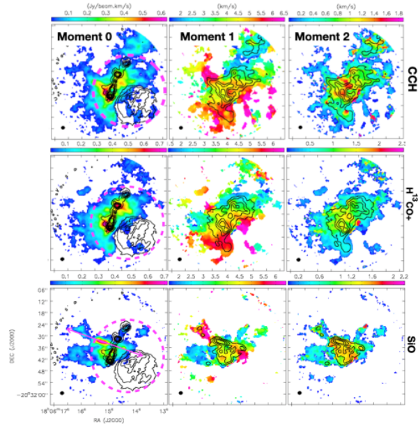
Figure A2. The images and contours are same as in Figure A1. The peak integrated intensities ( F_{\text{peak}} ) for CCH, \text{H}^{13}\text{CO}^+ and SiO are 0.63, 0.75, and 0.72 \text{Jy beam}^{-1} \text{km s}^{-1} , respectively. The magenta dashed circle on the Moment 0 maps show the clump boundary traced by \text{H}^{13}\text{CN} . The magenta arrow represents the direction of the bipolar outflow driven by MM6.
