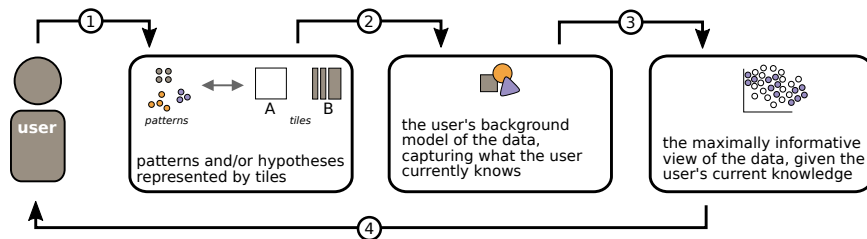
Figure 1: Overview of the exploration framework. (1) The user inputs his or her current knowledge and exploration objectives. (2) A background distribution, which captures what the user currently knows is constructed. (3) The most informative view of the data with respect to the background distribution and the user’s objectives is computed. (4) The user observes the data in the view, recognises relations and inputs these into the background distribution. The iterative data analysis process continues from (1).
