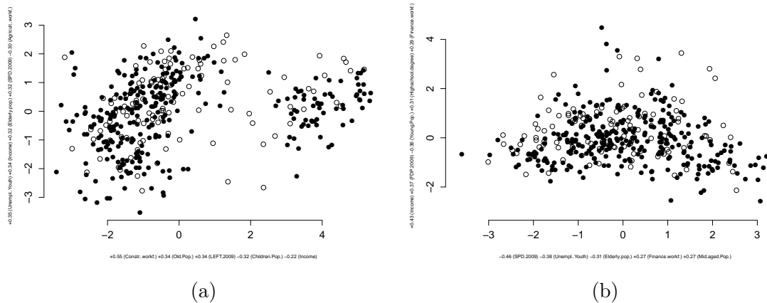
Figure 12: Views of the GERMAN data set corresponding to the hypothesis pairs (a) \mathcal{H}_{F,\emptyset} and (b) \mathcal{H}_{F,\{t\}} . Data points inside the focus area are shown using filled circles ( \bullet ) and points outside the focus area are shown using hollow circles ( \circ ). The x and y axis labels show the five attributes with the largest absolute values in each projection vector.
