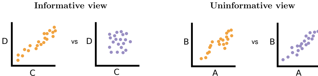
Figure 3: Two data samples (shown in orange and purple) in two projections. A view is informative if the data samples differ, which means that the user can learn something new about the data. In the left view the data samples differ with respect to the attributes C and D and the view is informative. In contrast, in the right view the data samples are essentially the same and the user learns nothing new about the relation between attributes A and B , and consequently the view is uninformative.
