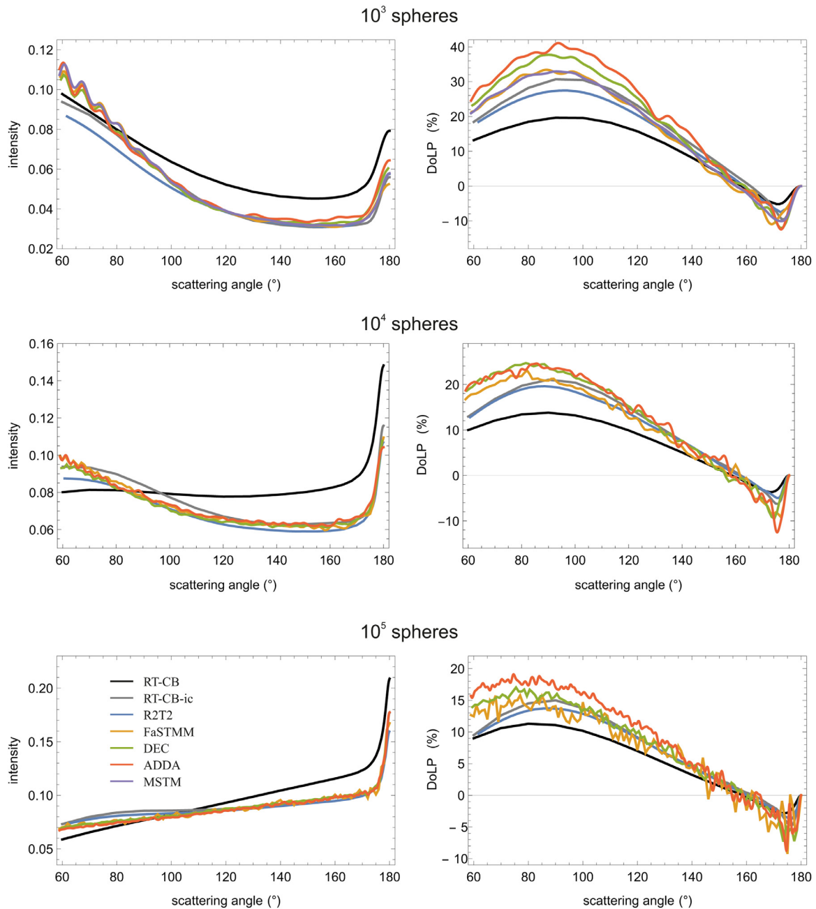
Fig. 2. The intensity and the degree of linear polarization computed with the available codes for the spherical volume containing variable amount of spherical particles in \nu = 20\% packing density. Continues in Fig. 3.
