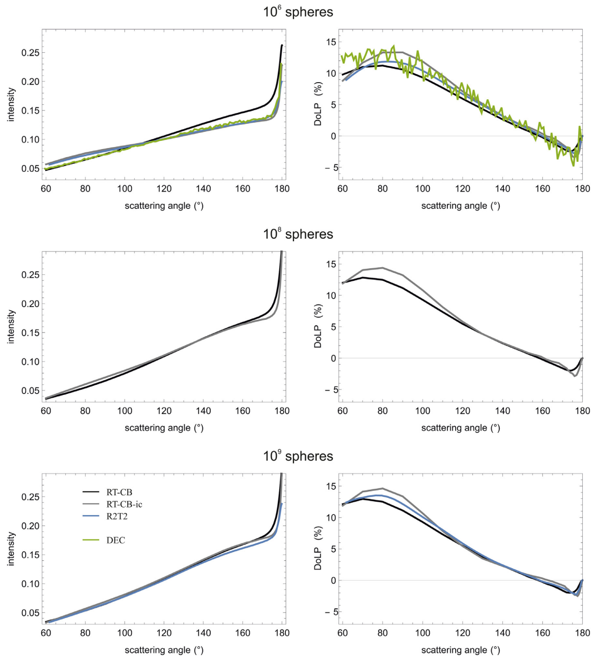
Fig. 3. Continued from Fig. 2.
