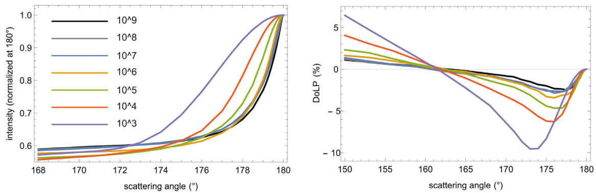
Fig. 5. The scattering phase function (in the left) and the degree of linear polarization (in the right) for backscattering region. Results are computed with the RT-CB-ic method. The plot legend panel indicates the powers of ten for the number of particles in the target.
