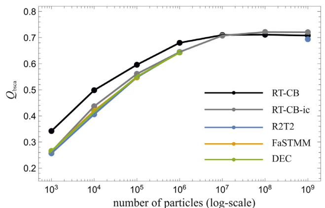
Fig. 4. The backscattering hemisphere scattering efficiency Q_{bsca} as a function of the target size, expressed as the number of particles in the cloud. The Q_{bsca} is shown here for five methods, of which the FaSTMM and DEC rigorously solve the macroscopic Maxwell equations, and the RT-CB, RT-CB-ic, and R^2T^2 are based on the radiative transfer approximation. The results with ADDA go up to 10^5 particles and MSTM to 10^3 particles, they follow the same overall trend but are not shown here.
