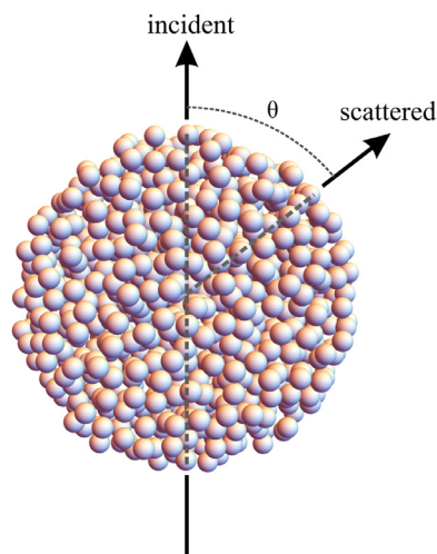
Fig. 1. One random realization of 10^3 equal-sized spheres that are packed in a spherical volume with 20% packing density. The scattering angle \theta is the angle between the direction of the incident field and the observing direction of the scattered field.
