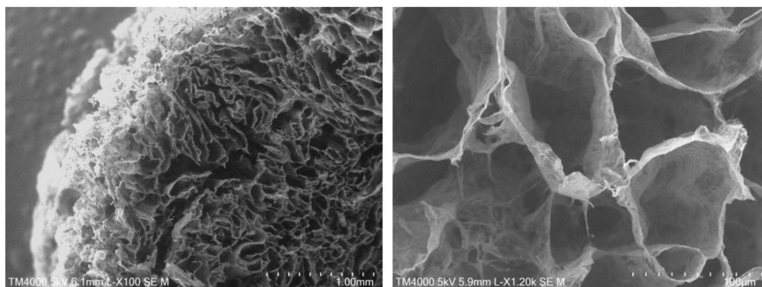
Figure 1. SEM (scanning electron microscopy) images of GO-PEI macrostructure obtained after lyophilization evidencing the porous nature of this materials.
