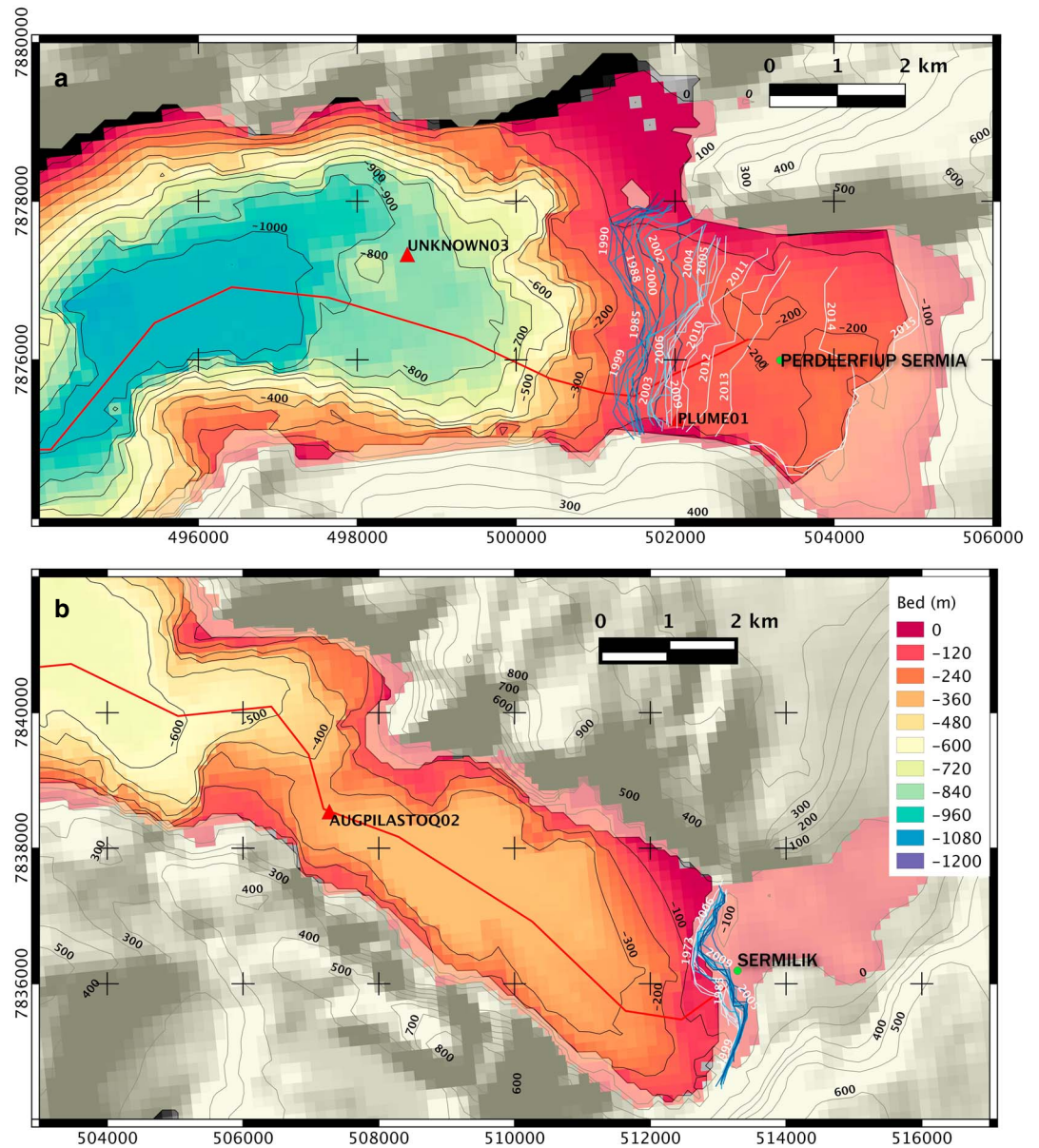
Figure 3. Bathymetry from MBES data with 100 m contour levels in (a) Perdlerfiup Fjord and (b) Sermilik Fjord showing glaciers grounded in shallow waters in otherwise deep (>800 m) fjords. CTD locations from year 2013 are red triangles with name in black. Red line denotes the profile used in Figure 2. Bed elevation (same color code) inland of the calving front is from Morlighem et al. [2014]. Ice front positions from 1964 to 2015 are color coded from blue to white and labeled by year.
