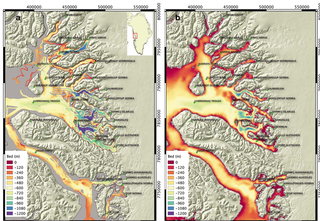
Figure 1. Bathymetry of Uummannaq and Vaigat fjords, west Greenland from (a) multibeam echo sounding data (MBES) acquired in 2007–2014 and (b) IBCAO3 [Jakobsson et al. , 2012] with bed elevation color coded from red (sea level) to blue (<−1200 m). Land ice mask (shaded) is from 2007. Glacier, fjord, and island names are black. Grey denotes no bathymetry data. Inset shows location in Greenland. UTM zone 22 unit in meters.
