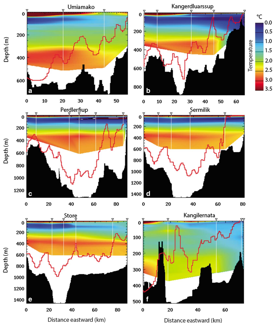
Figure 2. Bathymetry from MBES data (in black) acquired in 2012–2014 starting from the west moving east toward the glacier fronts, with IBCAO3 bed elevation in red, and potential temperature from CTD color coded from blue (0°C) to red (+3.5°C) going from north to south with (a) Umiamakko Isbrae, (b) Kangerdluassup Sermerssua, (c) Perdlerfiup Sermia, (d) Sermilik, (e) Store, and (f) Kangilerngata with CTD cast location as triangle. White denotes no temperature data.
