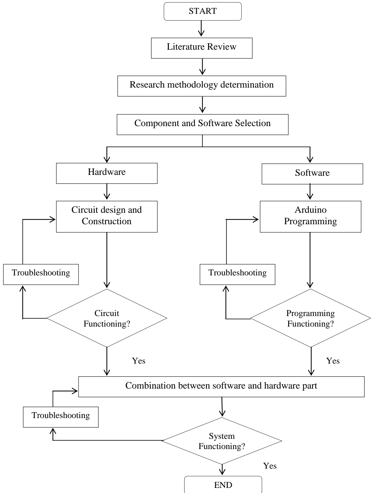
Figure 3.1: Methodology flowchart
