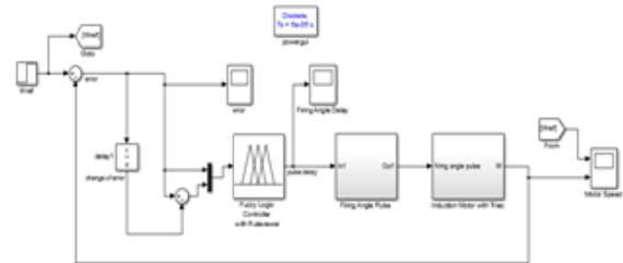
Figure-5. Fuzzy logic controller model in Simulink.
