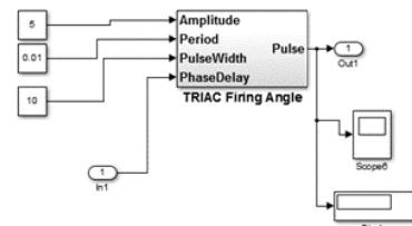
Figure-6. Triac firing pulse subsystem.
