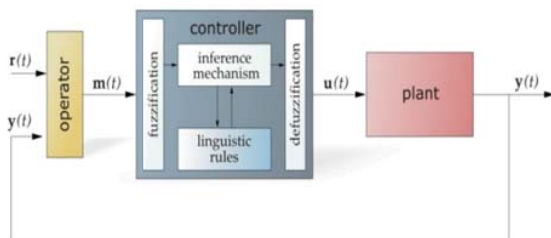
Figure-3. A typical fuzzy control system schema.
