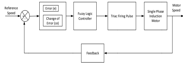
Figure-4. Block diagram overall the single phase induction motor speed control using fuzzy logic controller.
