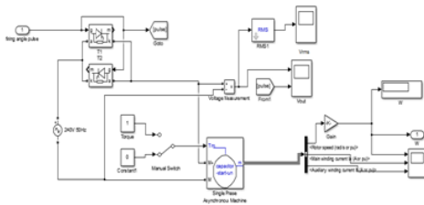
Figure-8. Simulink model for single phase induction motor with triac.
