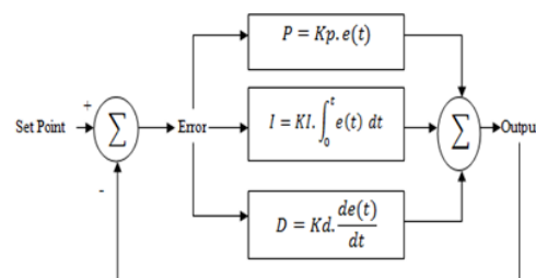
Figure-2. Block diagram of PID controller
