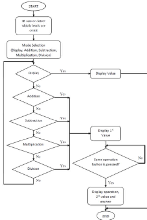
Figure 1: Flowchart of E-Abacus
