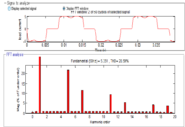
Figure 12: THD without SAPF
