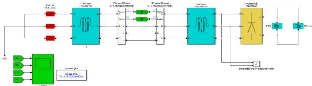
Figure 5: First simulation setup in MATLAB/Simulink with nonlinear load
