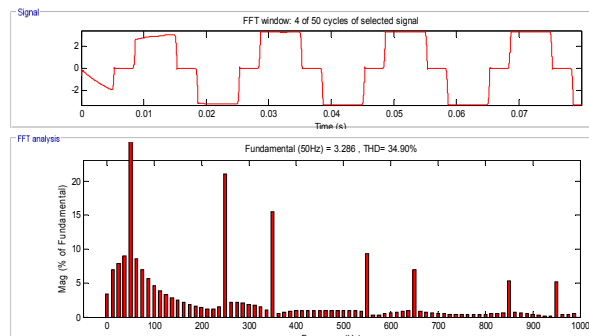
Figure 20: Analysis of THD without SAPF
