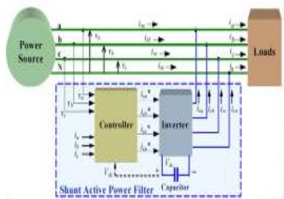
Figure 4: SAPF in 3-phase system (Priya and Balu, 2014)
