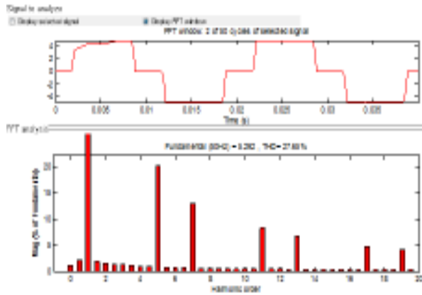
Figure 16: An analysis of THD without SAPF
