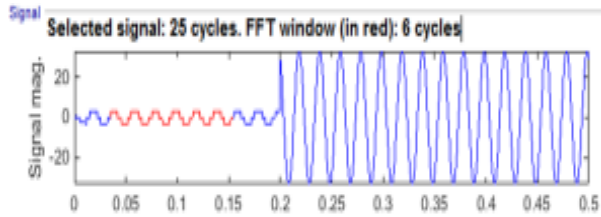
Figure 15: Current waveform without SAPF
