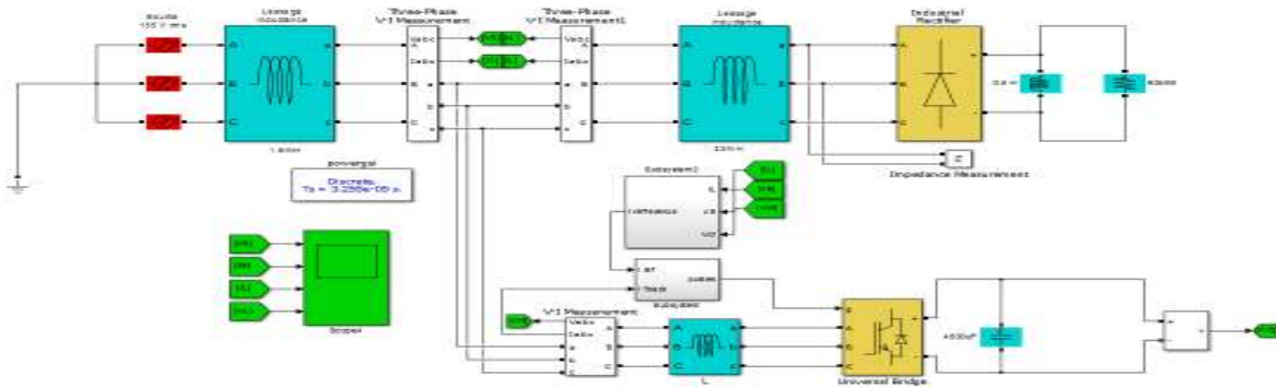
Figure 6: Second simulation setup with SAPF
