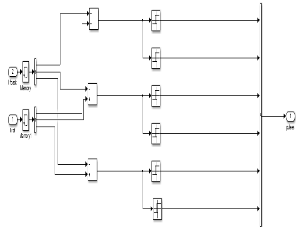
Figure 8: Hysteresis current control
