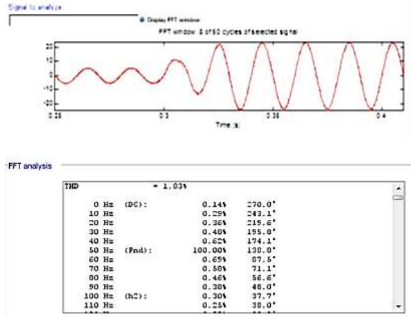
Figure 18: Analysis of THD with SAPF
