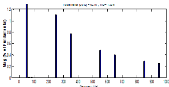
Figure 24: Analysis of THD with SAPF
