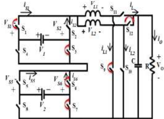
Figure 3: Derivation circuit of the mode 1
