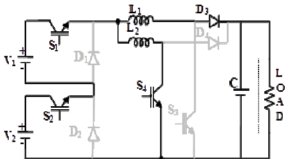
Figure 10: Operating mode-2 at time T_2 .
