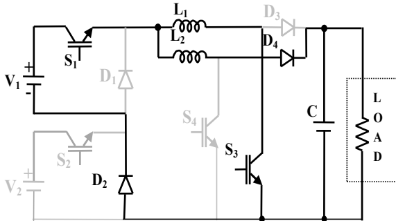
Figure 9: Operating mode-1 at time T_1 .
