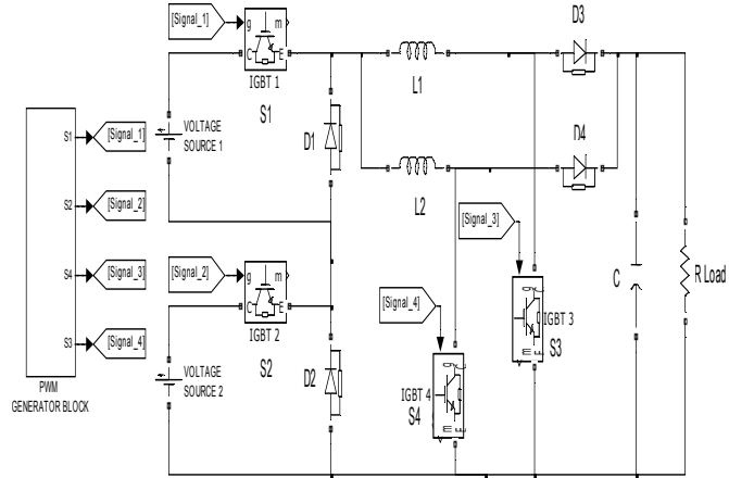
Figure 13: Simulation model circuit of proposed multi-input interleaved boost converter
