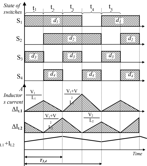
Figure 8: Pulse modulation of the switches and current waveforms of the proposed multi-input converter.
