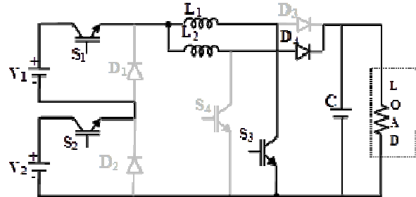
Figure 11: Operating mode-3 at time T_3 .
