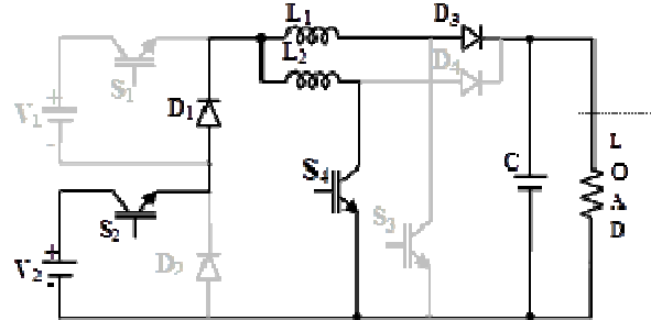
Figure 12: Operating mode-4 at time T_4 .
