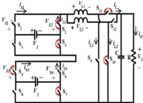
Figure 6: Derivation circuit of the mode 4
