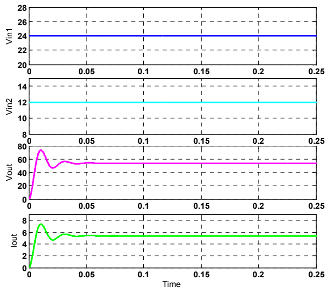
Figure 17: Voltage input sources ( V_{in1} and V_{in2} ); output voltage V_{out} ; output current I_{out}
