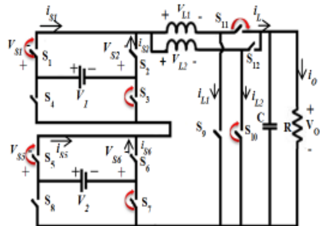
Figure 4: Derivation circuit of the mode 2
