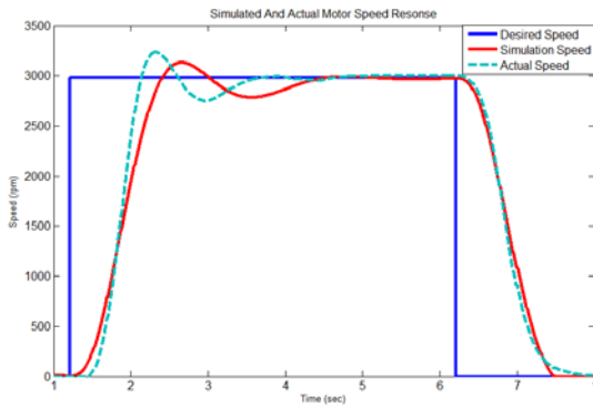
Figure 14 : Comparison of simulation and Actual speed
