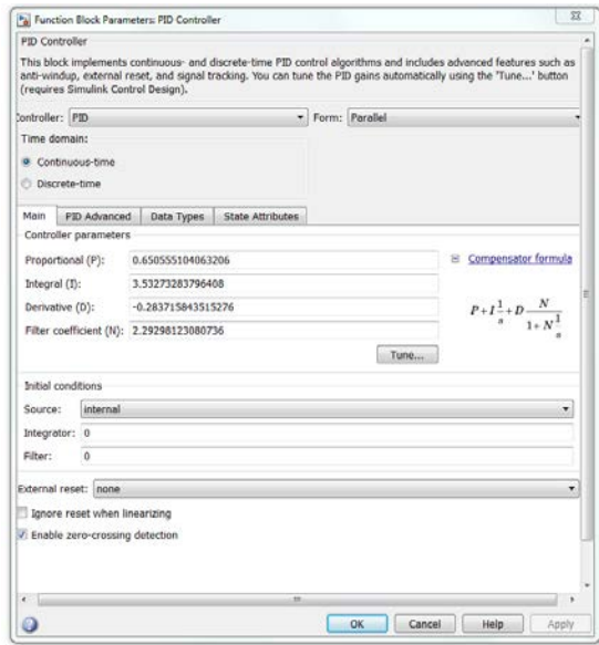
Figure 10: PID Controller Auto tuning GUI
