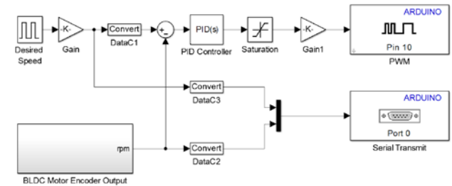
Figure 12: Simulink model of Arduino Mega program for PID controller
