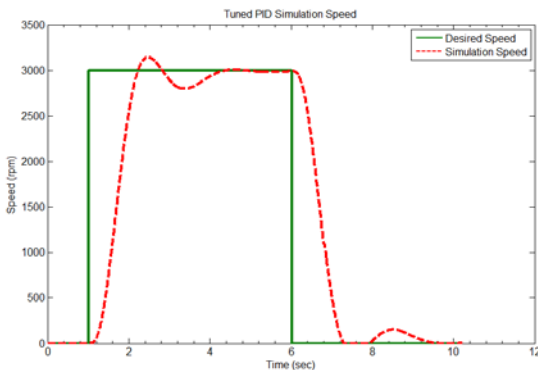
Figure 11: Simulation of PID controller model response
