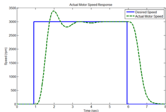
Figure 13: Actual motor speed in closed-loop
