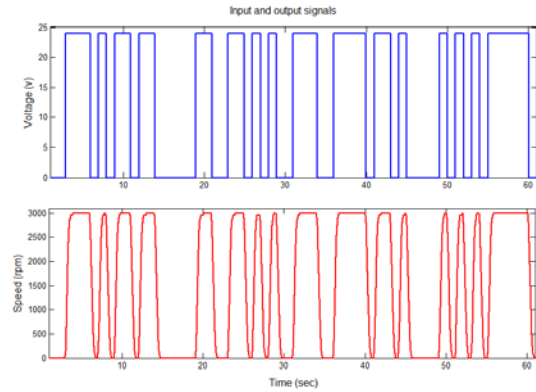
Figure 6: PRBS and motor speed signal captured in MATLAB
