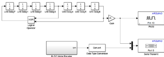
Figure 5 : PRBS generator simulink model
