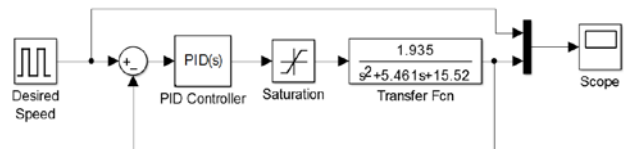
Figure 9: System model for BLDC motor control
