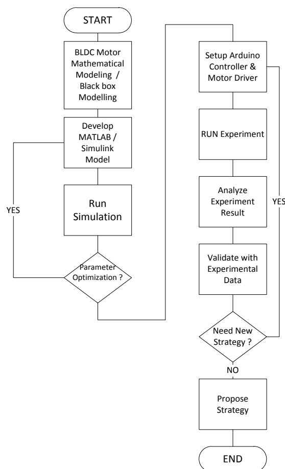
Figure 1: Design Flow of Model-Based Design
