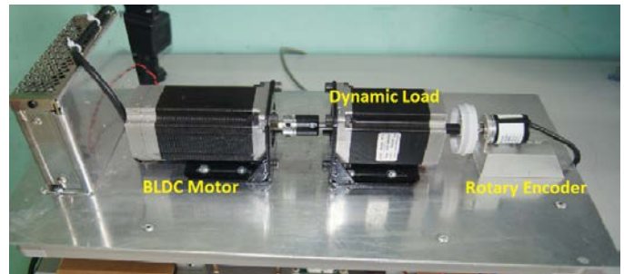
Figure 2 : BLDC Motor Plant
