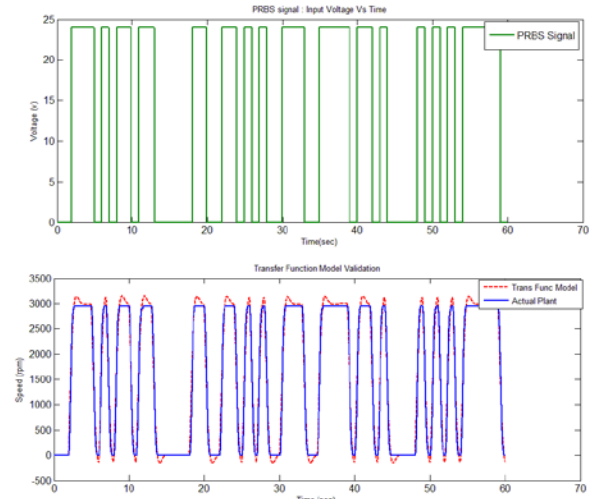
Figure 8: Transfer function model validation
