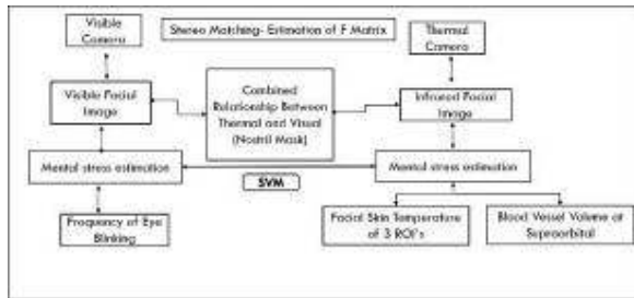
Figure 1: Overall System.
