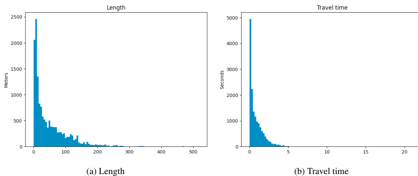
Fig. 2: Histogram of the variables length and travel time of the bicycle network in the city center of Amsterdam
