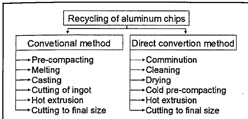
Figure 1.2: A comparison of conventional and direct recycling techniques of Aluminium alloy chip (Tekkaya et al. , 2009)
