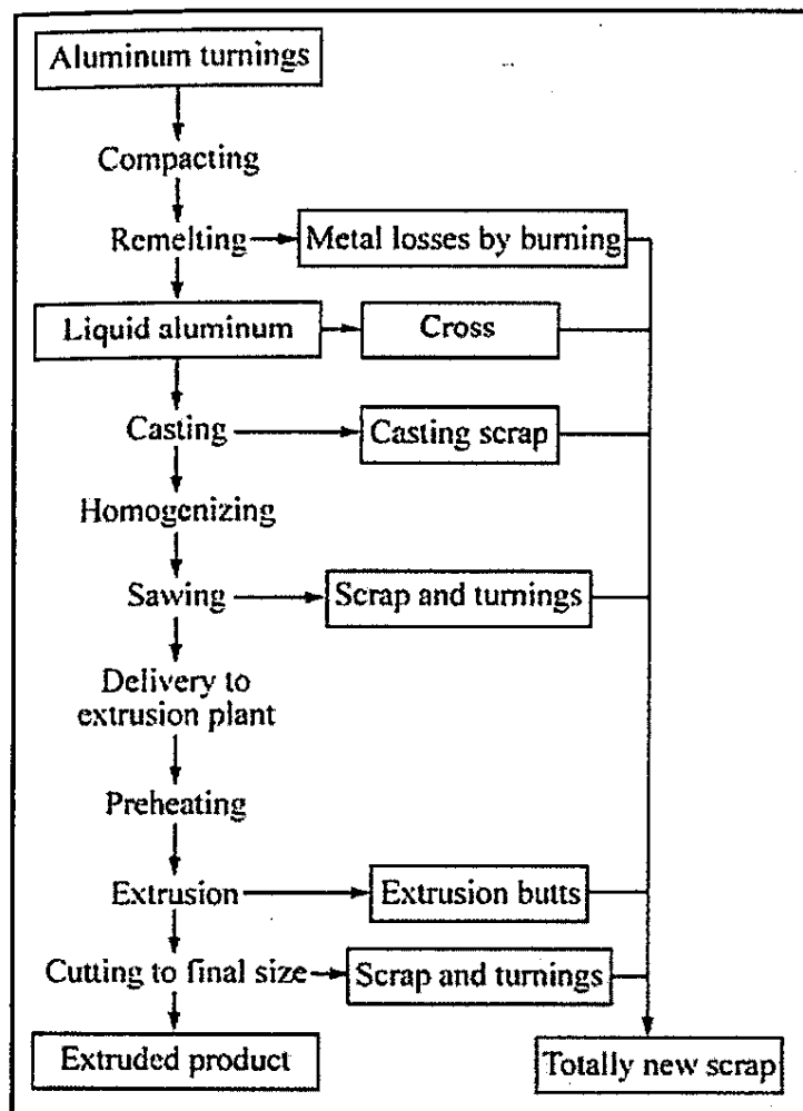
Figure 1.3: Flow chart of conventional process for recycling of aluminum turnings (Jirang and Hans, 2010)
