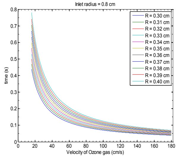
Fig. 6: Internal diameter (R =0.30 - 0.40 cm) for 50cm gas cell with an inlet radius of 0.8 cm
