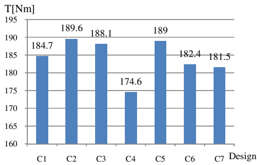
Fig. 3. The maximum torque for all configurations
