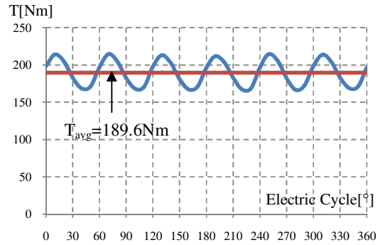
Fig. 4. Instantaneous torque for C2
