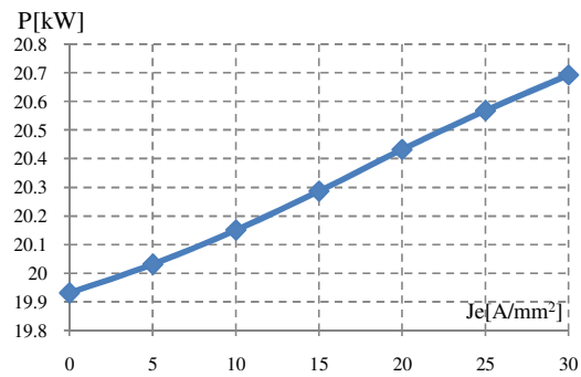
Fig. 6. Power vs various J_e at maximum J_a for C2
