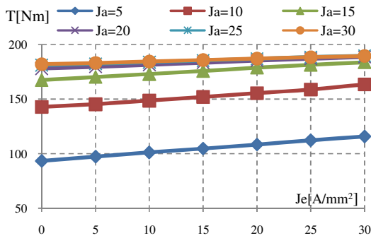
Fig. 5. Torque vs J_e at various J_a for C2
