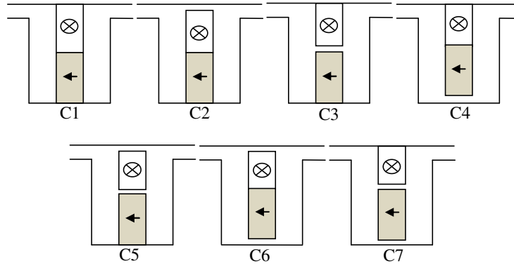
Fig. 2. The arrangement of iron flux bridges
