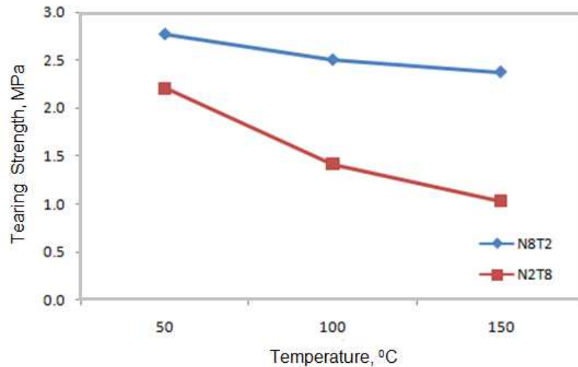
Fig. 6 Effect of heat compression on tearing strength
