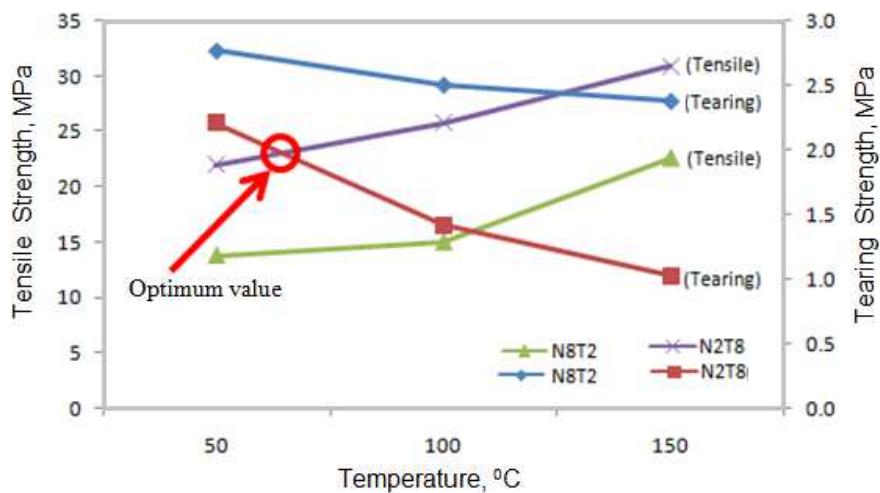
Fig. 7 The optimum heat compression on tensile and tearing strength
