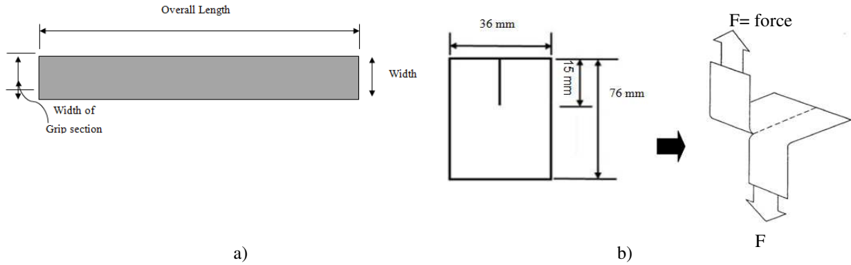
Fig. 4 Specimens geometry for a) Tensile test b) Tearing test
