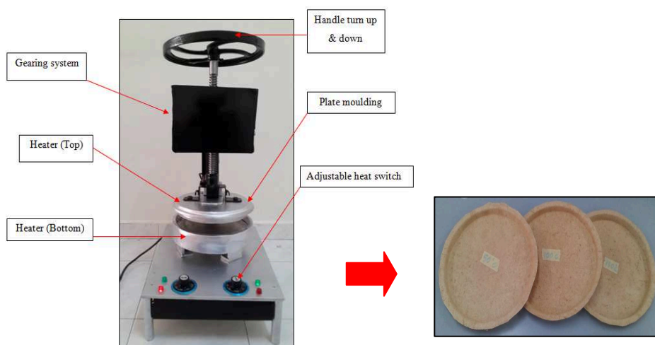
Fig. 3 Hot press machine for disposable plate producing
