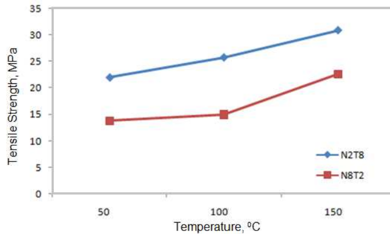
Fig. 5 Effect of heat compression on tensile strength
