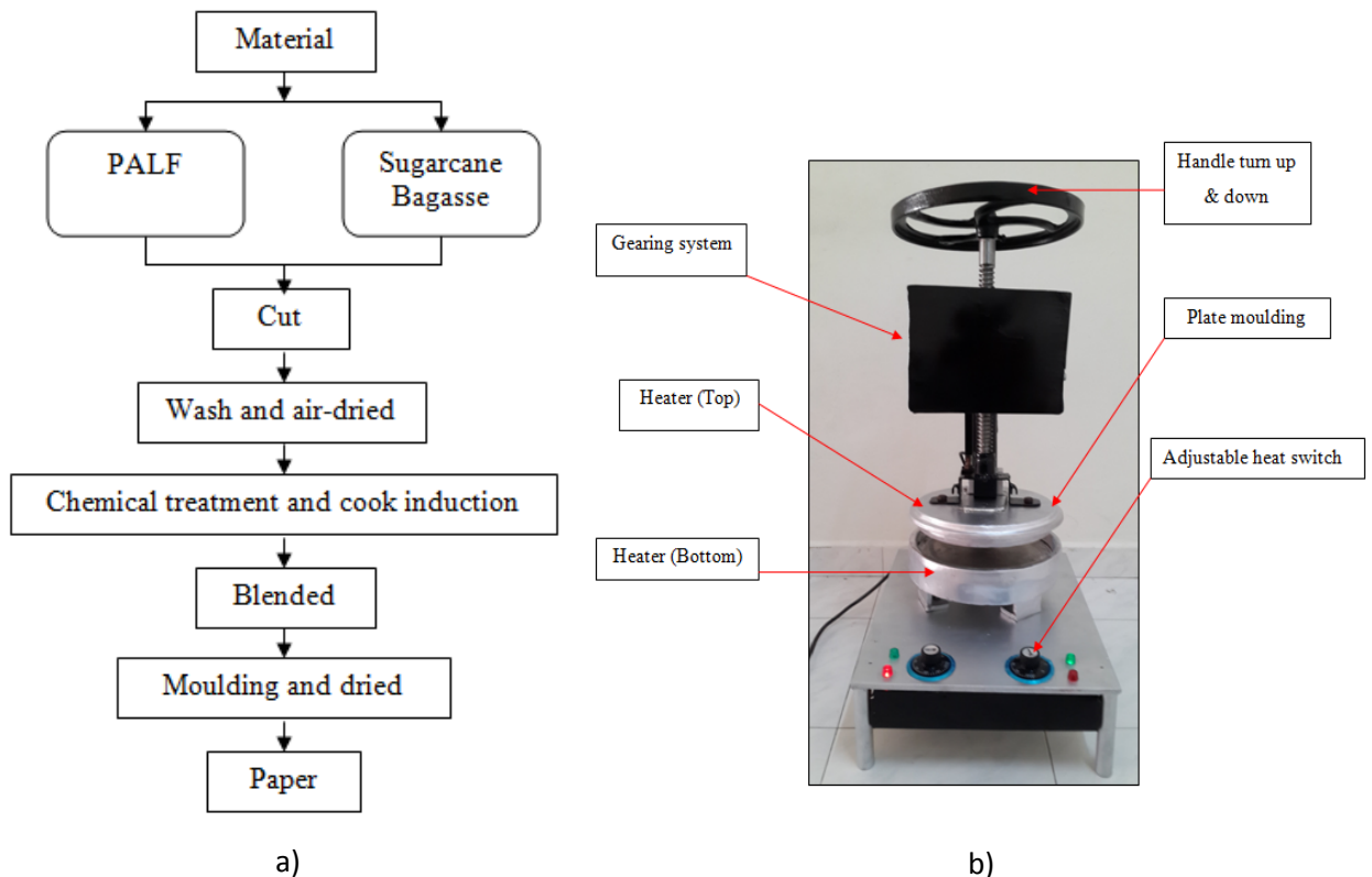
Figure 1: a)Schematic Specimen preparation b) Hot press machine for disposable plate producing
