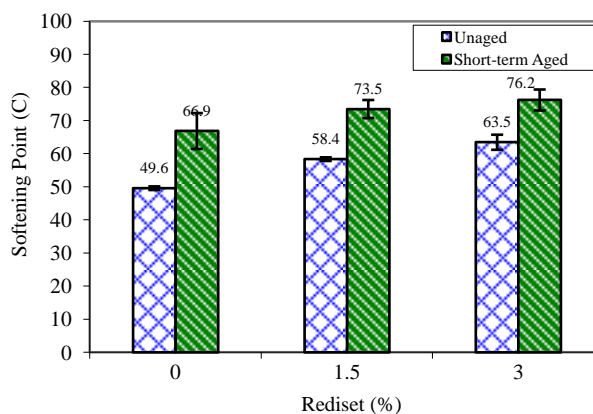
Figure 2 Effects of Rediset ® on aging state conditions
