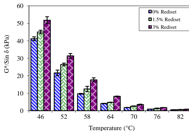
Figure 4 G*/Sin δ of short-term aged at different temperatures
