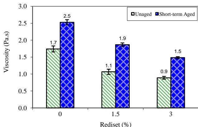
Figure 3 Viscosity of unaged and short-term aged binder containing Rediset® at 135°C
