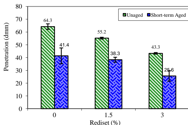
Figure 1 Penetration of binders containing Rediset ® for unaged and short-term aged
