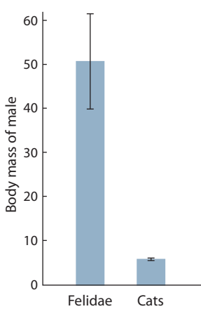
Fig. 3. A comparison of mean maximum male body mass, its range and standard deviation in wild Felidae and domestic cats.
