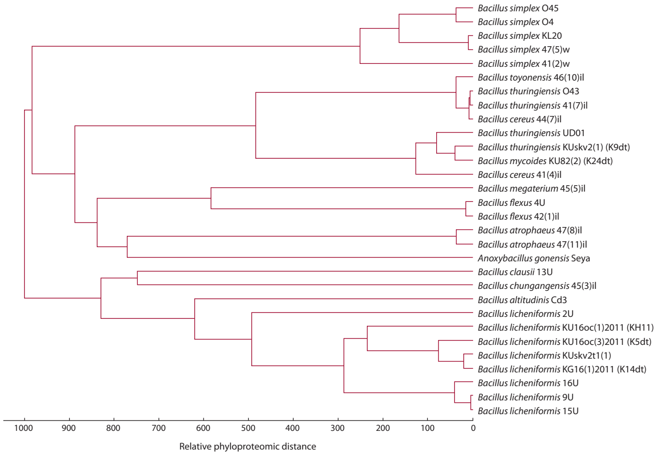
Fig. 2. Phyloproteomic tree constructed with Biotyper 3 for characteristic mass spectra of strains studied.
