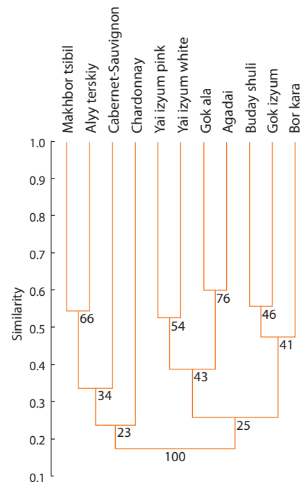
Fig. 1. Dendrogram of the genetic similarity of grapevine cultivars on the base of SSR data.
