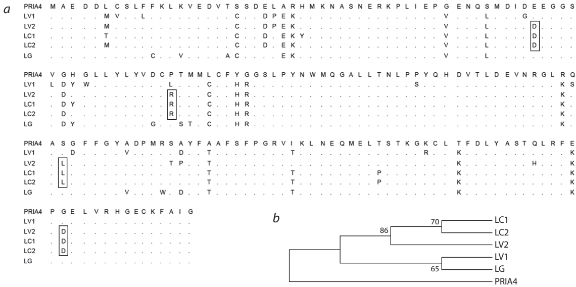
Fig. 1. Comparison of RoIC amino acid sequences from A. rhizogenes A4 (PRIA4), the left and right borders of cT-DNA from L. vulgaris (LV1 and LV2, respectively), L. genistifolia (LG), and L. cretica (LC1 и LC2). (a) Alignment of amino acid sequences. Boxes indicate amino acids matching in LV2, LC1, and LC2 but differing in other sequences. (b) Phylogenetic tree constructed by the maximum likelihood method. The consensus tree is constructed from 500 bootstrap replicates. The starting tree for heuristic search was constructed by the neighbor-joining and BioNJ methods applied to the matrix of pairwise distances assessed by the JTT model and subsequent choice of tree topology with larger likelihood logarithms.
