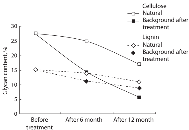
Variation of cellulose and lignin contents in corn crop residues after treatments with a granulated lab specimen (LS, G) based on T. asperellum G-034 strain (substrate multirecycled with Shiitake-Oyster mushrooms) at the application rate 10 g/m 2 .
