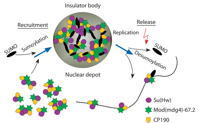
Fig. 4. The model describing the organization of insulator bodies (reproduced from (Golovnin et al., 2012)).
