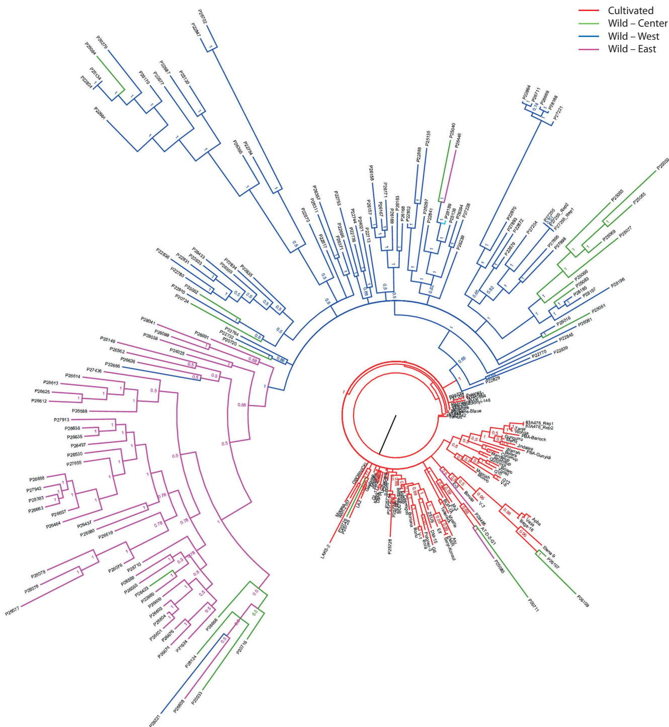
Fig. 1. The phylogenetic tree for wild and cultivated narrow-leaved lupine accessions produced on 11,690 SNPs using MrBayes v3.2.2, according to (Mousavi Derazmahalleh et al., 2018).
