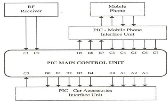
Fig. 7. PIC Based MCCS Schematic Diagram
