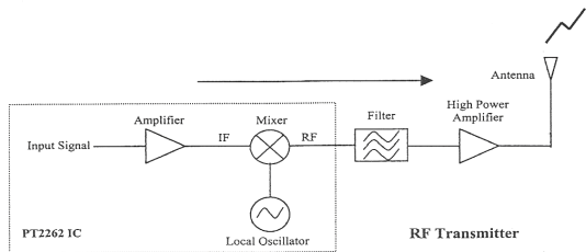
Fig. 9a. Block diagram of RF Transmitter
