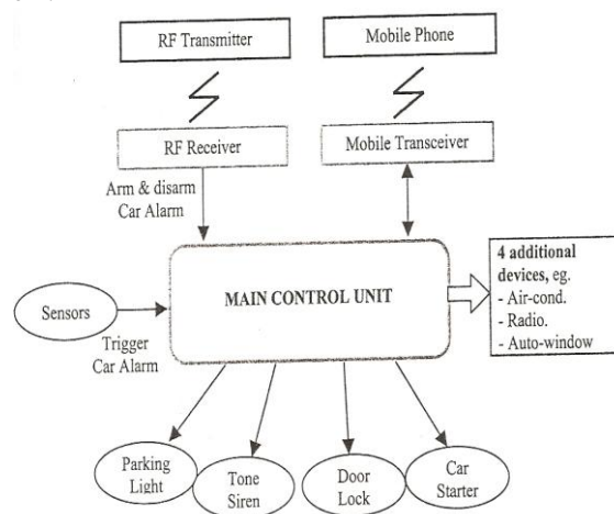
Fig. 1. MCCA System Configuration
