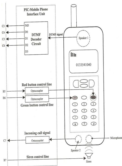
Fig. 12 Circuit Connections to the mobile phone
