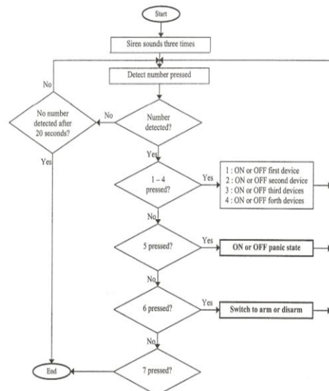
Fig. 21. The program logic in the phone control state
