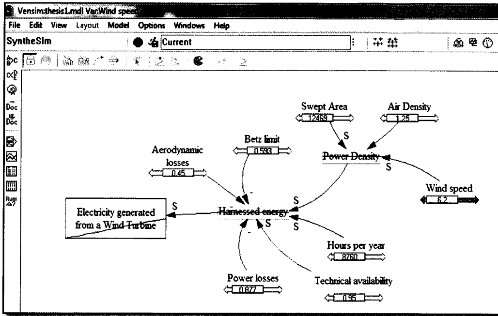
Fig. 11. Simulation on change for the electricity generation flow diagram. Source: Author's construction based on VENSIM software.
