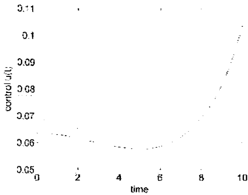
Figure 4 – Control v time shooting algorithm.
