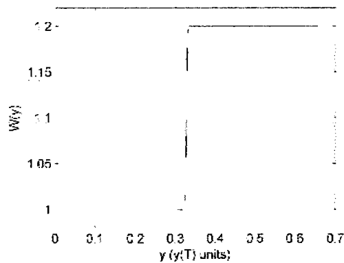
Figure 1 W(y) approximation.
