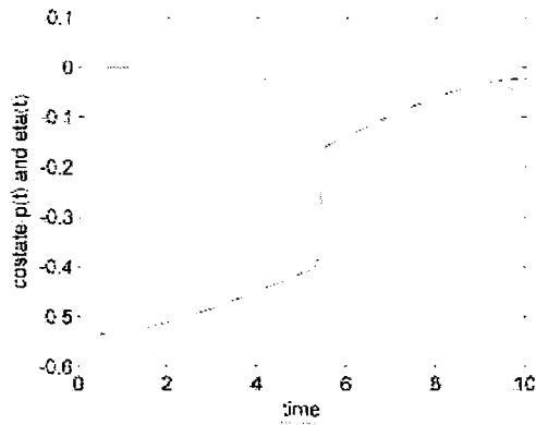
Figure 3 – Costate v time shooting algorithm.
