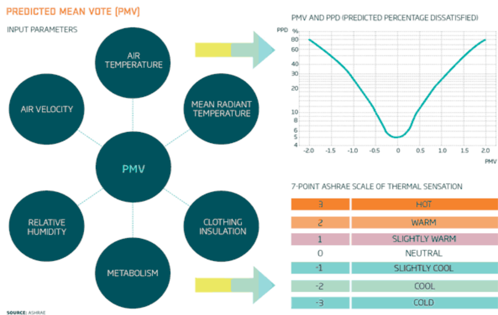
Figure 2.7: PPD as a function of PMV (ASHRAE-55, 2004)
