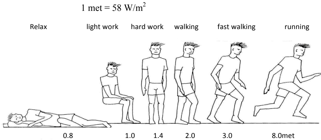
Figure 2.5: Metabolic rate of different activities (Fanger P. O., in: “Energy and Building” 3/1985)
