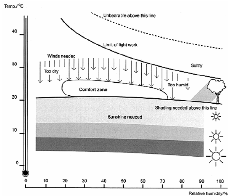
Figure 2.8: Bioclimatic chart (Olgay Victor, 1963)
