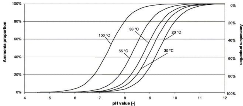
Figure 4. \text{NH}_3/\text{NH}_4^+ equilibrium curve for varying pH and temperature. Taken from (Fricke, et al., 2007 with calculations from Kollbach, et al., 1996)
