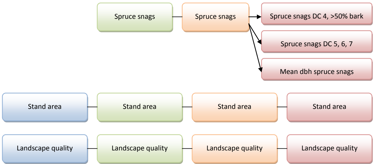
Figure 4- The four hypotheses and their explanatory variables included in the global model addressing each of them. The letters “DC” mean “decay class”.
