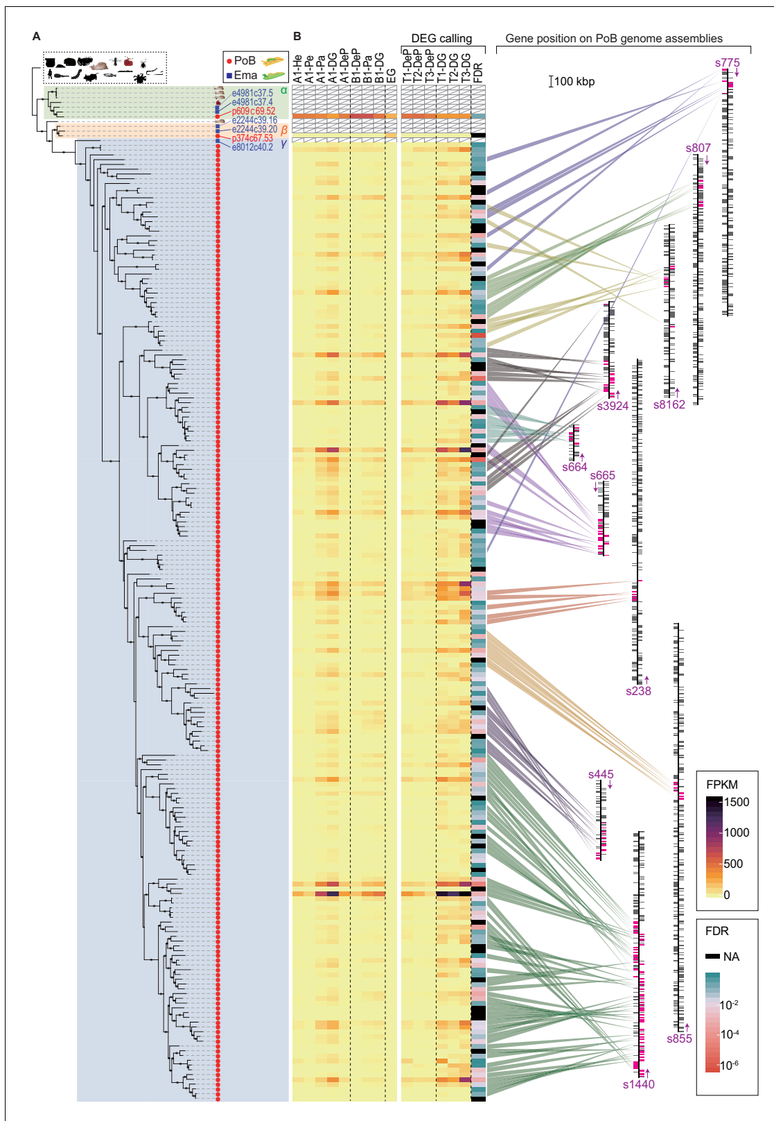
Figure 6. Evolutionary process of KRM gene candidates of OG0000132. (A) ML phylogenetic tree for OG0000132 genes (for details, see Figure 6—figure supplement 1 ). Red circle, PoB gene; blue square, E. marginata (Ema) gene. Genes mentioned in the text are indicated with their IDs beside the circles. Pictograms represent non-sacoglossan species defined in Figure 5—source data 2 . (B) Expression of each PoB gene and gene position on the genomic assemblies. The left-side heat plot indicates normalized expression degree (FPKM) of the PoB genes in various tissues; tissue abbreviations Figure 6 continued on next page
