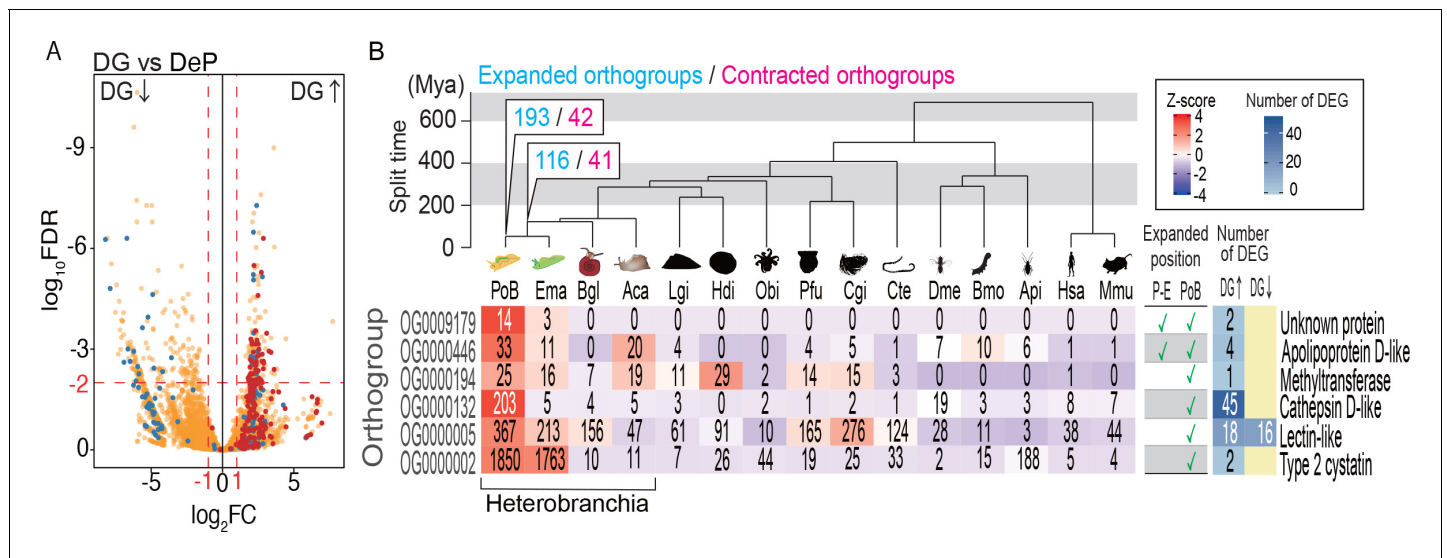
Figure 5. Probable KRM genes in PoB. (A) Volcano plot comparing gene expressions in DG and DeP tissues of PoB. Red, orthogroup OG0000132 (cathepsin D-like protease genes); blue, orthogroup OG0000005 (lectin-like genes); orange, other orthogroups (for details, see Figure 5—figure supplement 2 ). Up and down arrows signify up- and down-regulation, respectively, in DG. (B) Orthogroups expanded on the P. ocellatus lineage and containing DG-up-regulated genes. Ema, E. marginata ; Bgl, B. glabrata ; Lgi, Lottia gigantea ; Hdi, Haliotis discus ; Obi, Octopus bimaculoides ; Pfu, Pinctada fucata ; Cgi, Crassostrea gigas ; Cte, Capitella teleta ; Dme, D. melanogaster ; Bmo, Bombyx mori ; Api, A. pisum ; Hsa, Homo sapiens ; Mmu, Mus musculus . The phylogenetic tree was scaled to divergence time based on 30 conserved single-copy genes. Mya, million years. The numbers of rapidly expanded (blue) and contracted (magenta) orthogroups on the lineages to PoB are provided at the nodes (for details, see Figure 5—figure supplements 4 and 5 ). Below the tree is information for the six expanded orthogroups that contained DG-up-regulated genes. The left-side heatmap shows the gene numbers (number in boxes) and Z-score of gene numbers (color gradient) for each orthogroup. The table shows the expanded/not expanded status of each orthogroup (P-E, Plakobranchus-Elysia node; PoB, Plakobranchus node). The right-side heat map indicates the number of DEGs between DG and DeP tissue in each orthogroup. Representative gene products are given on the far right. The source files of RNA-Seq analysis and comparative genomic analysis are available in raw data Figure 5—source data 1 and 2 , respectively. The online version of this article includes the following source data and figure supplement(s) for figure 5:
