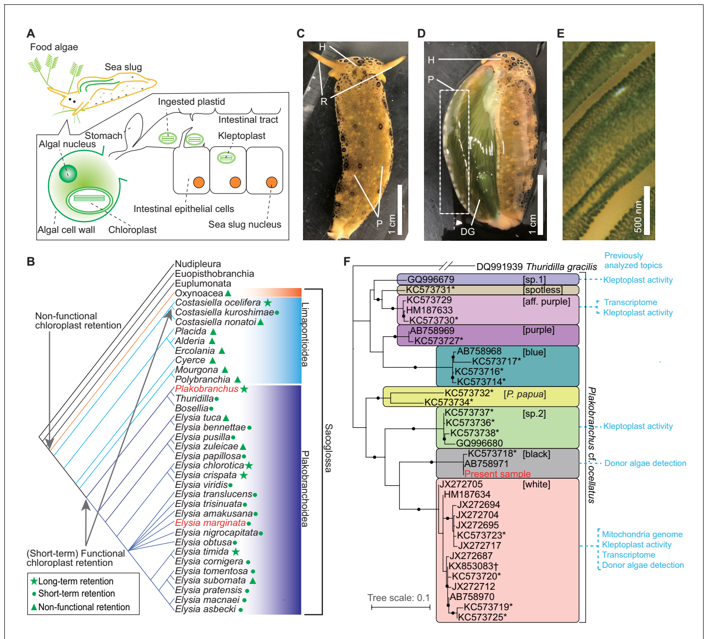
Figure 1. Kleptoplasty in sea slugs. (A) Process of algal chloroplast retention by a sacoglossan sea slug (Pierce and Curtis, 2012). Sacoglossan sea slugs puncture the cell wall of food algae to suck out the protoplasm. The chloroplasts in the protoplasm are transported to the sea slug’s intestinal tract, and the intestinal epithelial cells sequester chloroplasts by phagocytosis. The sequestered chloroplasts (kleptoplasts) maintain the photosynthetic activity in the cell for days to months. The sacoglossan cell contains no algal nuclei. Kleptoplast has never been found in germ cells of sea slug. (B) Phylogenetic distribution of kleptoplasty in the order Sacoglossa. Phylogenetic analysis showed that a common ancestor of Sacoglossa acquired non-functional chloroplast retention phenomena (without the maintenance of photosynthetic function), and multiple sacoglossan groups subsequently acquired the ability to maintain photosynthetic activity. Phylogenetic tree and kleptoplasty states are simplified from Christa et al., 2015. Christa et al., 2014b defined functional chloroplast retention for less than 2 weeks as ‘short-term retention’, and for more than 20 days as ‘long-term retention’. Relationships within Heterobranchia are described according to Zapata et al., 2014. The red-colored taxa include the species used in the present study ( P. ocellatus and E. marginata ). (C–E) Photo images of PoB starved for 21 days. (C) Dorsal view. H, head; R, rhinophores; P, parapodia (lateral fleshy flat protrusions). Almost always, PoB folded parapodia to the back in nature. (D) The same individual of which parapodium was turned inside out (without dissection). The back of the sea slug and inside of the parapodia are green. This coloration is caused by the kleptoplasts in DG, which are visible through the epidermis. (E) Magnified view of the inner surface of parapodium. The diagonal green streaks are ridged projections on the inner surface of the parapodium. The cells containing kleptoplasts are visible as green spots. (F) Phylogeny of the P. cf. ocellatus species complex Figure 1 continued on next page
