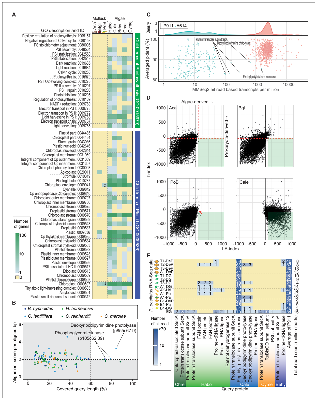
Figure 4. Search for horizontally transferred algal genes in the PoB genome. (A) Heatmap of the number of genes assigned to photosynthesis- or plastid-related GO terms. The abundance of photosynthesis- or plastid-related genes was compared among PoB, two non-kleptoplatic mollusk species ( Aca , A. californica ; Bgl , B. glabrata ), and five algal species (see abbreviations in Figure 3 , Figure 3—source data 1 ). A color scale was visualized in the box on the left. (B) Scatter plot of the Exonerate results, the alignment of the A614 gene set (query sequences) to the PoB genome. Figure 4 continued on next page
