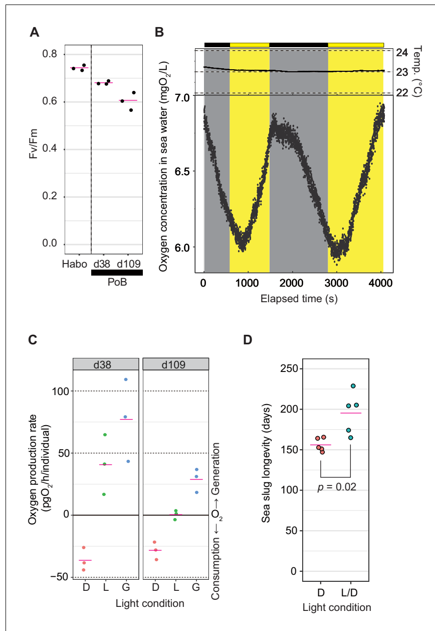
Figure 2. Photosynthetic activity of PoB. (A) Jitter plot of Fv/Fm values indicating the photochemical efficiency of PSII. Habo, H. borneensis ; d38, starved PoB for 38 days; d109, starved for 109 to 110 days (12 hr light/12 hr dark cycle; the light phase illumination was 10 \mu\text{mol photons m}^{-2} \text{s}^{-1} ). The magenta line indicates the mean, and the black dot indicates each individual's raw value ( n = 3 per group). (B) Dynamics of seawater oxygen concentration. To better demonstrate the PoB photosynthesis, a change of oxygen concentration every second was visualized. A PoB individual, one of the d38 samples (ID1), was put into the measurement chamber, and the light conditions were changed in tens of minutes. The measurements in other individuals are visualized in Figure 2—figure supplement 1 , along with the diagrams of the measuring equipment. Each point represents the oxygen concentration value per second. Gray signifies a dark period, and yellow means an illuminated period (50 \mu\text{mol photons m}^{-2} \text{s}^{-1} ). Temp, water temperature. Although the values fluctuated by the noise due to ambient light and other factors, the oxygen concentration decreased in the dark conditions and increased in the light conditions. When the illumination condition was changed, the changing pattern kept the previous pattern for a few minutes. This discrepancy may reflect the distance between the organism and oxygen sensor and the time for adaptation to brightness by the kleptoplast. (C) Jitter plots of PoB oxygen consumption and generation. D, dark conditions; L, light conditions; G, gross rate of light-dependent oxygen generation (L minus D). (D) Jitter plots of PoB longevity ( n = 5 per group). D, Continuous dark; L/D, 12 hr light/12 hr dark cycle. The p from Welch's two-sample t-test was p = 0.02 . Figure 2 continued on next page
