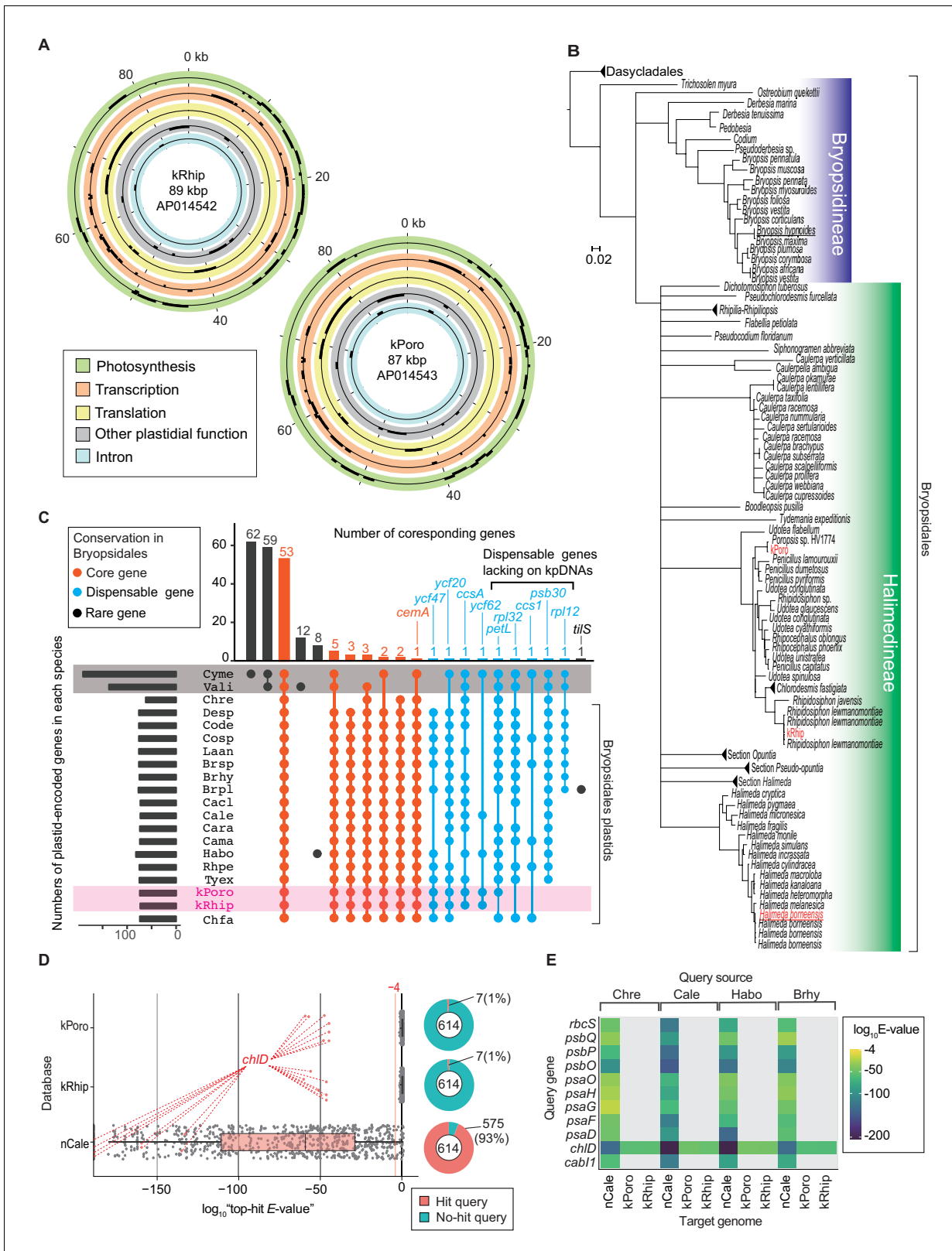
Figure 3. Gene composition of PoB kpDNAs. (A) Gene map of two kpDNAs from PoB. Gene positions are described in circles colored according to the gene's functional category (see keys in the box). Genes on the outside and inside of each circle are transcribed in the clockwise and anticlockwise directions, respectively (for detailed maps, see Figure 3—figure supplements 1 and 2 ). (B) Phylogenetic positions of sequenced kleptoplasts among green algal plastids. The original ML tree ( Figure 3—figure supplement 4 ) was created based on rbcl genes (457 positions) and converted to the tree. Figure 3 continued on next page
