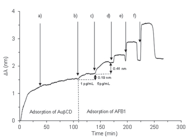
Figure 5. SPR curve of AFB1 (b) 1, c) 5, d) 30, e) 30, f) 60 pg/mL) on a) Au \beta CD NPs modified surface measured on SPR platform (acetonitrile content was \sim 2 ppm in every sample)
