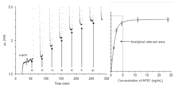
Figure 4. SPR curve of AFB1 (b) 1, c) 5, d) 10, e) 30, f) 60 \mu\text{g/ml} on a) Au \beta CD NPs modified surface measured on SPR platform, and adsorption isotherm of AFB1 on Au \beta CD NP-modified Au film measured on SPR platform
