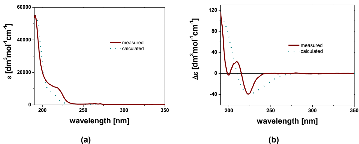
FIGURE 3 Calculated (dashed line) UV absorption (a) and CD (b) spectra of ( R )-4-chloro-1-phenyl-5-methyl-1,2,3,6-tetrahydrophosphinine 1-oxide [( R )-1] together with the measured (solid line) spectra of (+)-4-chloro-1-phenyl-5-methyl-1,2,3,6-tetrahydrophosphinine 1-oxide [(+)-1]. The solvent was acetonitrile.
