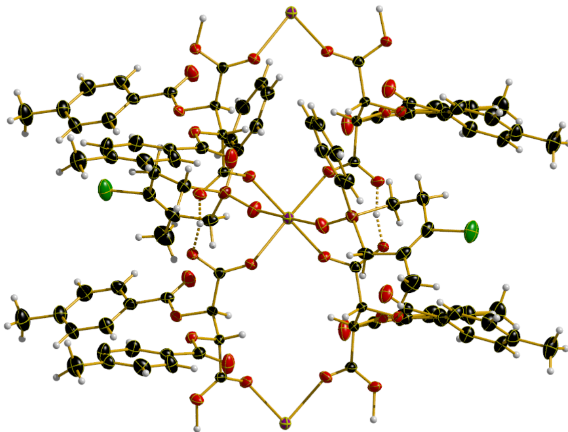
FIGURE 1 50% Atomic displacements plot of \text{Ca}(1)_2(\text{H-DPTTA})_2 showing carboxyl/carboxylate H-bridge contacts in broken lines. Disordered ethanol molecules are omitted for clarity from this drawing.
