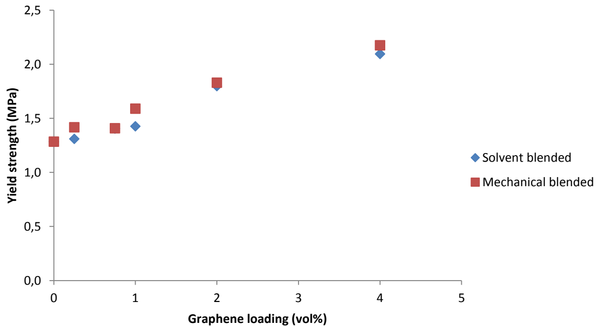
Figure 4: Inverse of Parameter b which denotes the yield strength of the powder blends
