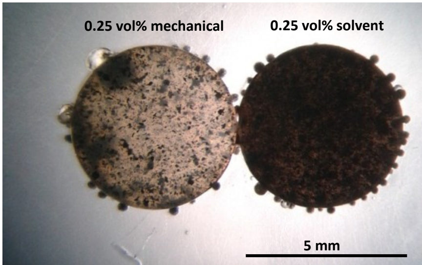
Figure 8: Micrograph of 0.25 vol% billets prepared by mechanical and solvent blended powders
