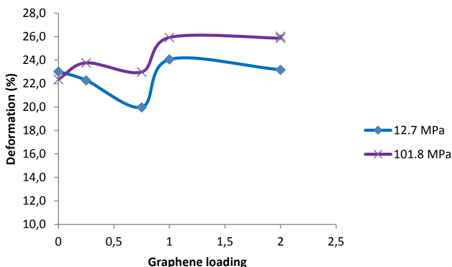
Figure 10: Deformation under load results for solvent blended samples
