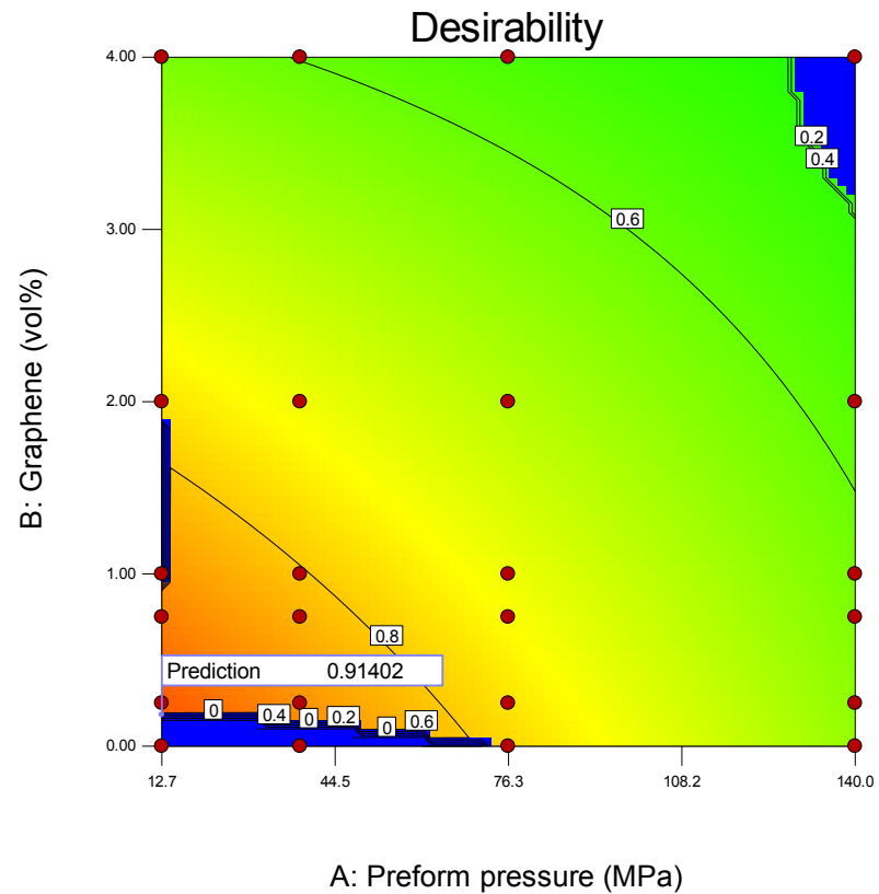
Figure 7: Prediction from design of experiments data
