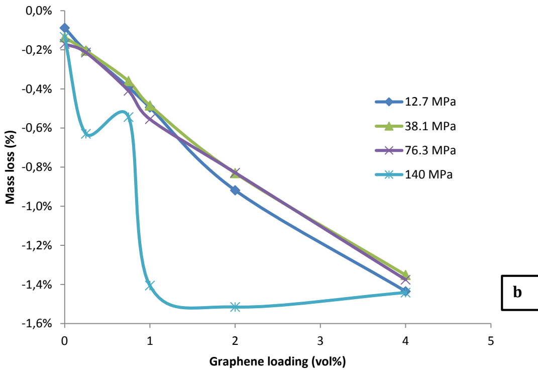
Figure 5: Change in mass of composite billets made with (a) solvent and (b) mechanical blended powders
