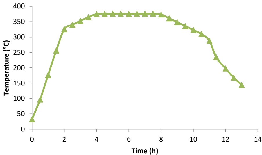
Figure 2: Sintering profile used to process the pre-form billets
