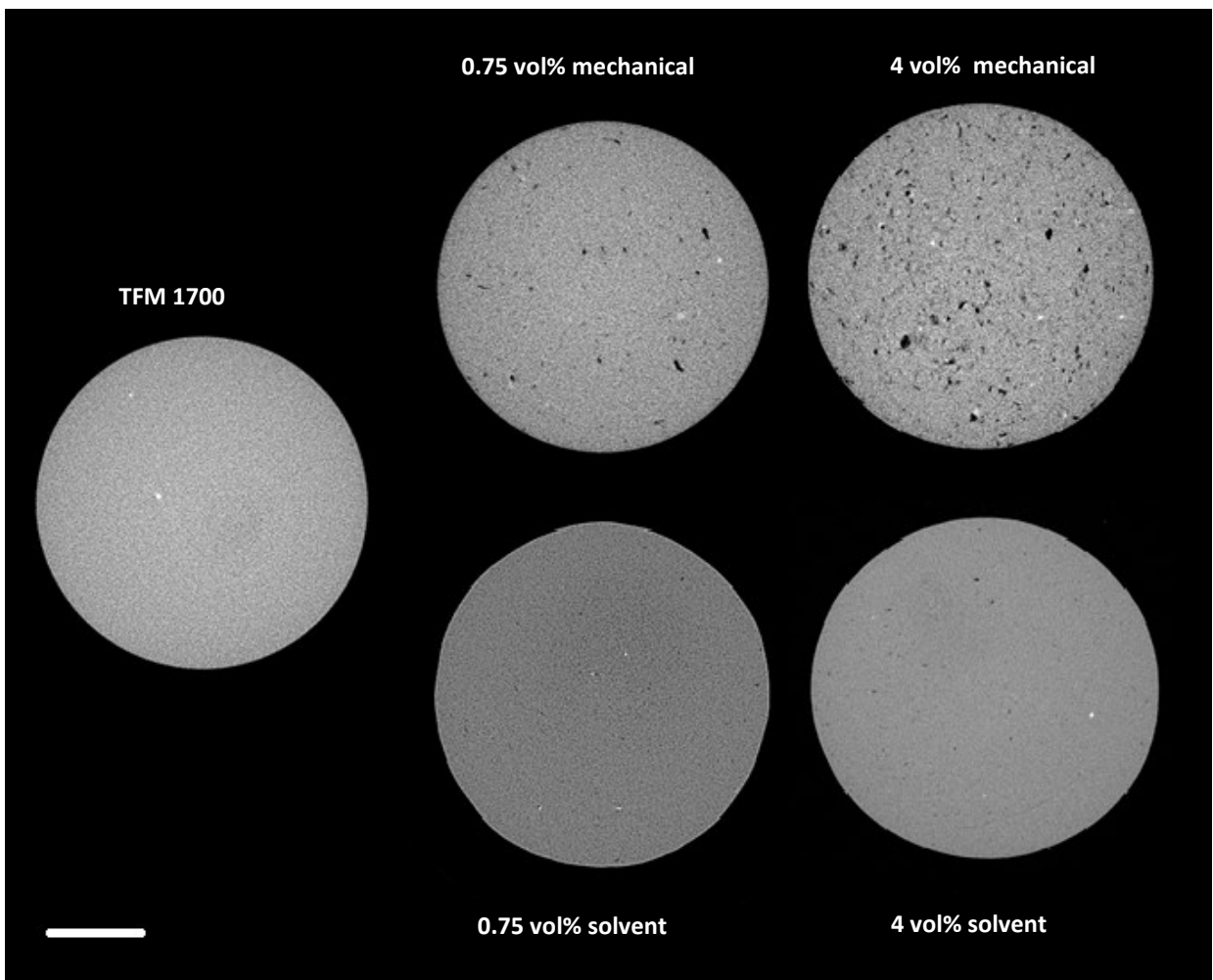
Figure 9: Micro CT slides of sintered mechanical and solvent blended billets prepared at a preform pressure of 12.7 MPa. The reference sample is also included for comparison reasons. Scale bar is 1.5 mm
