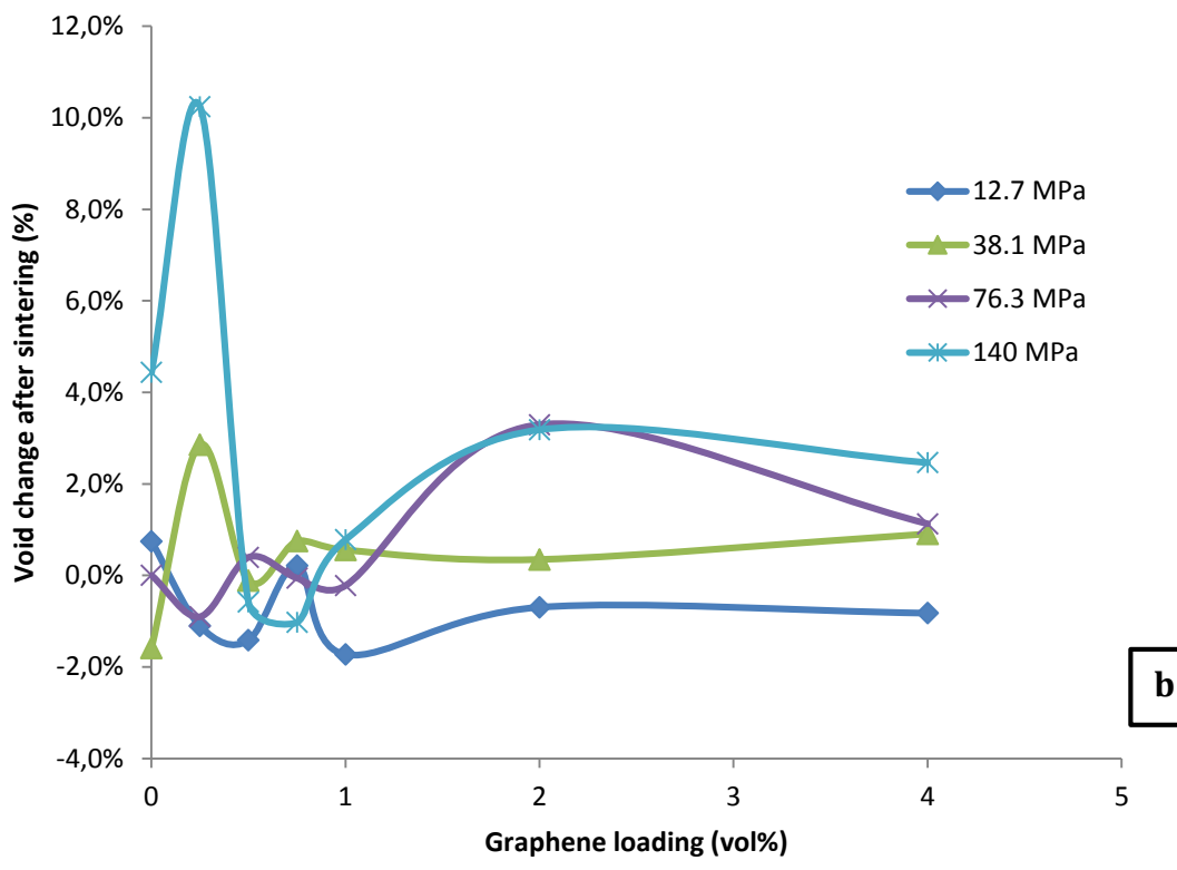
Figure 6: Void content of composite billets made with (a) solvent and (b) mechanical blended powders after sintering
