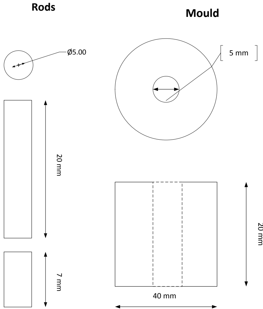
Figure 1: Drawing of stainless steel mould with base plate and plunger rods
