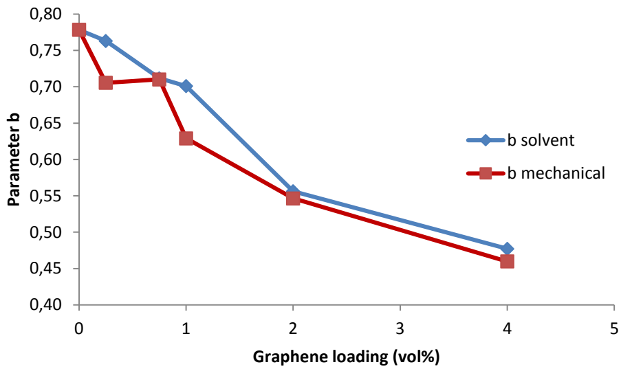
Figure 3: Influence of graphene on Kawakita parameters (a and b^{-1} ) for mechanical and solvent blended powders
