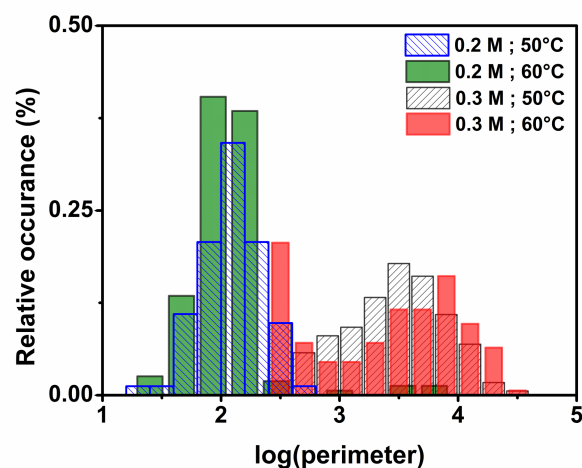
Figure 8. Effect of the different temperatures and ion concentration on the resulting clusters. The perimeter of the aggregates in nanometre was obtained from image analysis analysing 200 clusters.
