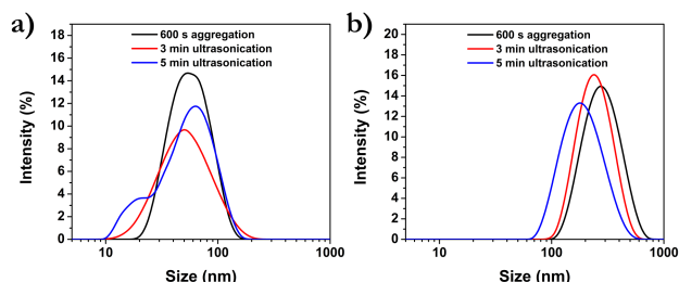
Figure 9. Effect of sonication on the DLS response for suspensions obtained after assembly for 600 seconds at (a) 0.2 M; 50 °C and (b) 0.3 M; 60 °C.
