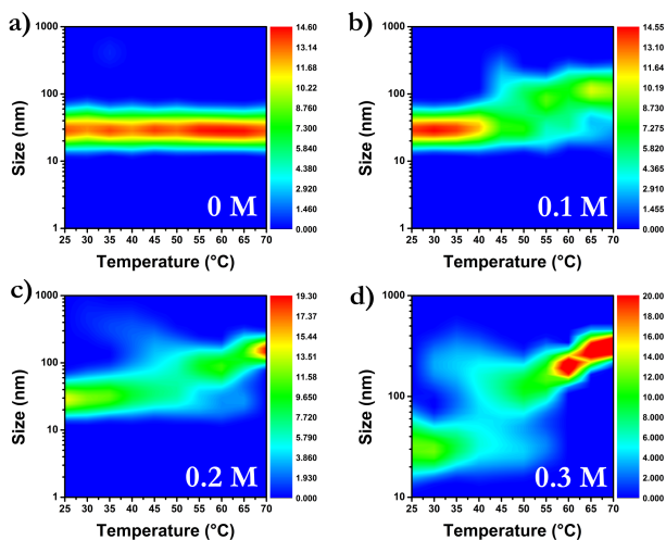
Figure 2. DLS size distribution as a function of temperature at different \text{K}_2\text{SO}_4 concentrations.
