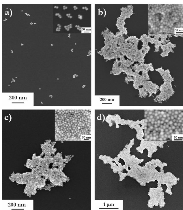
Figure 7. Structure of the gold nanoparticle clusters evolved after 40 minutes under different experimental conditions ( \text{K}_2\text{SO}_4 concentration and temperature): 0.2 M and 50 °C (a); 0.3 M and 50 °C (b); 0.2 M and 60 °C (c); 0.3 M and 60 °C (d). Insets show the compact alignment of nanoparticle building blocks.
