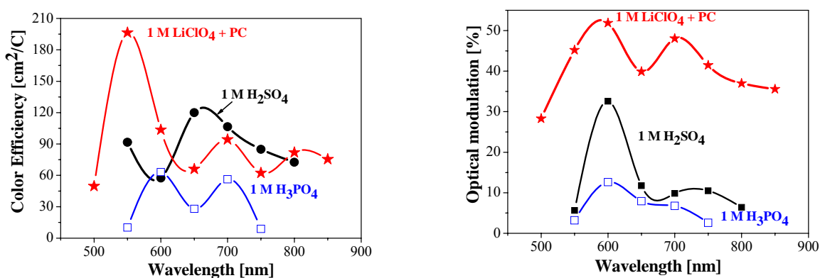
Figure 4. Electrochromic characteristics of CVD \text{MoO}_3\text{-WO}_3 films, derived from cyclic voltametric measurements in three types of electrolytes [37].
