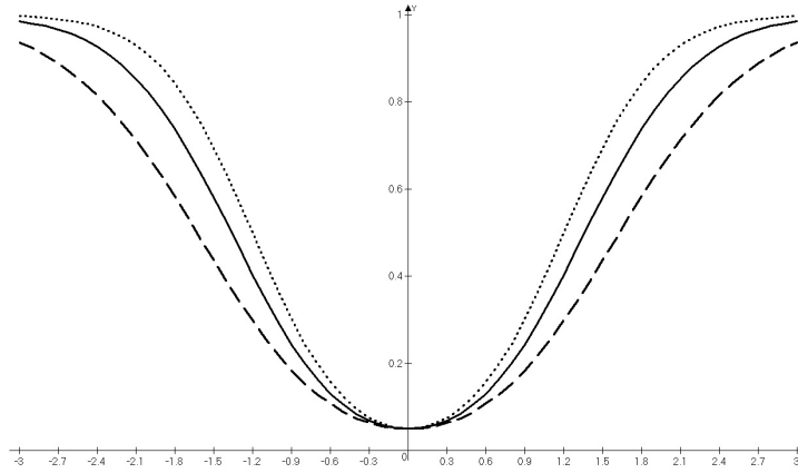
Fig. 1.4 Empirical power for \tilde{Q}_n with significance level 0.05, n = 400 (dashed), n = 600 (solid) and n = 800 (dotted) with k_1 = n/4
