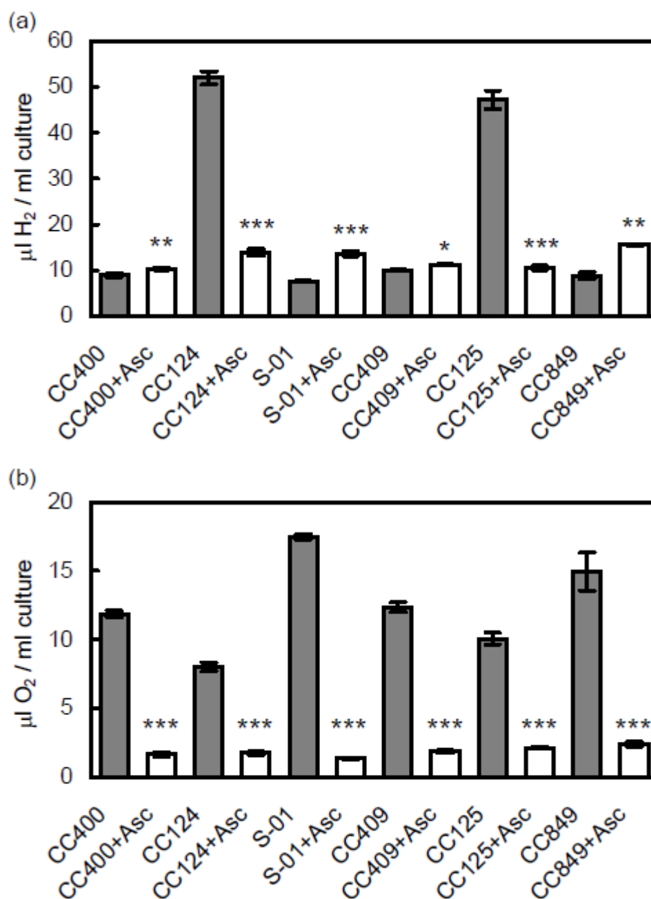
Figure 1. H 2 (A) and O 2 (B) accumulation by several C. reinhardtii strains without or with 10 mM Na-Asc added to the cultures at the start of sulphur deprivation. The amounts of H 2 and O 2 were determined daily by GC and the accumulated gases were removed by N 2 flushing after the measurements each day. Averages of the total H 2 and O 2 gases accumulated during four days, in three independent experiments are presented. Error bars represent standard errors and the significance level between the Asc-treated and untreated samples are presented as: * p<0.05; ** p<0.01;*** p<0.001.
