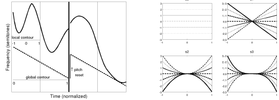
Figure 1: Left: CoPaSul stylization of global and local intonation components. Right: Variation of 3rd order polynomial coefficients to capture local contour shapes.
