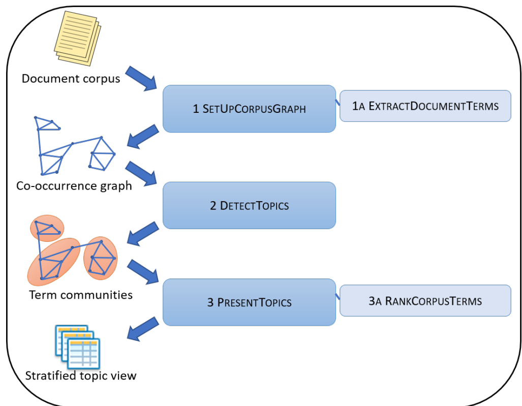
Figure 1. Workflow leading from a corpus of documents to a tabular presentation of topics. The various procedures involved in the workflow are described in detail in Sections 3.1–3.3.
