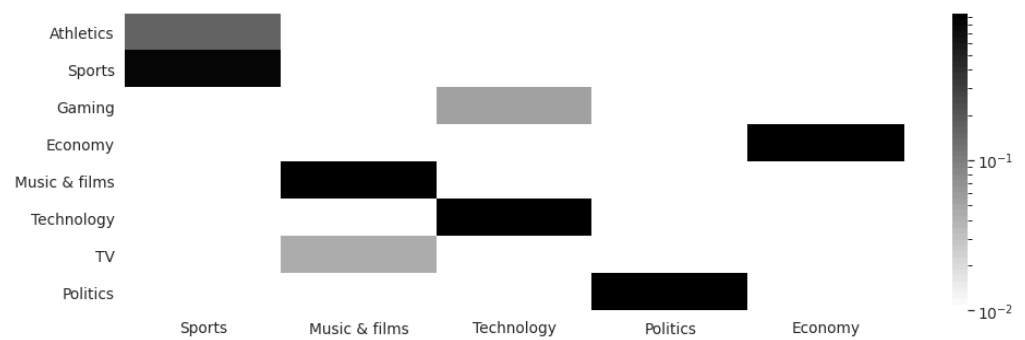
Figure 2. Heat map showing how topic terms of the 5 \gamma = 0.8 topics (columns) get distributed on 8 topics at \gamma = 1.0 (rows)
