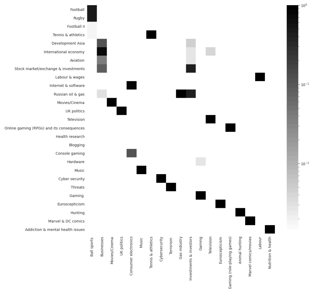
Figure 4. Heat map showing how topic terms of the 19 \gamma = 1.37 topics (columns) get distributed on 27 topics at \gamma = 1.5 (rows)
