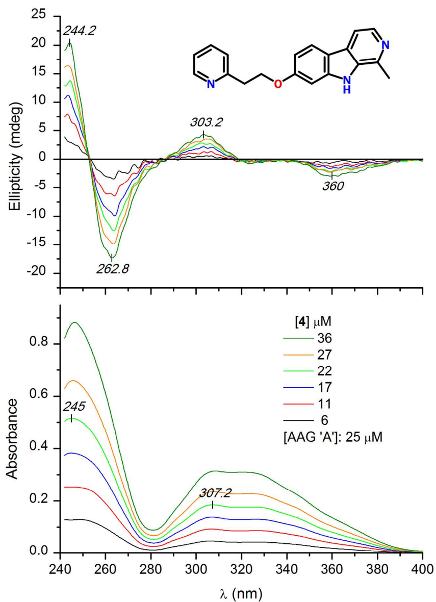
Figure 4. Difference CD and UV absorption spectra of compound 4 added to 25 μM buffer solution of the A genetic variant of AAG. 599x814mm (72 x 72 DPI)
