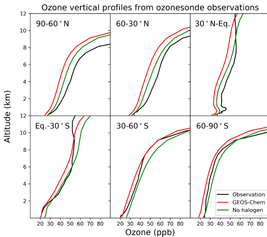
Figure 14. Annual average vertical profile of ozone mixing ratios from ozonesonde observations and the model for six zonal bands.
