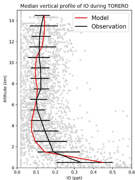
795 Figure 11. Median vertical profile of IO mixing ratios from the TORERO (Jan-Feb 2012 over the eastern tropical Pacific) campaign. Observations are shown as individual 1 min data points, with medians and 25th–75th percentiles in 1km vertical bins. Model values are shown as medians sampled along the flight tracks.
