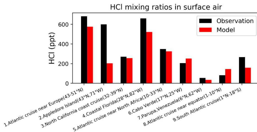
760 Figure 6. Surface air mixing ratios of HCl at coastal and island sites and from ocean cruises, arranged from left to right in order of decreasing latitude. Observations (black) are means or medians depending on availability from the publications. Model values (red) are monthly mean values in 2016 taken for the same month and location as the observations. References: (1, 5, 8, 9) Keene et al. (2009); (2) Keene et al. (2007); (3) Crisp et al. (2014); (4) Dasgupta et al. (2007); (6) Sander et al. (2013); (7) Sanhueza and Garaboto (2002).
