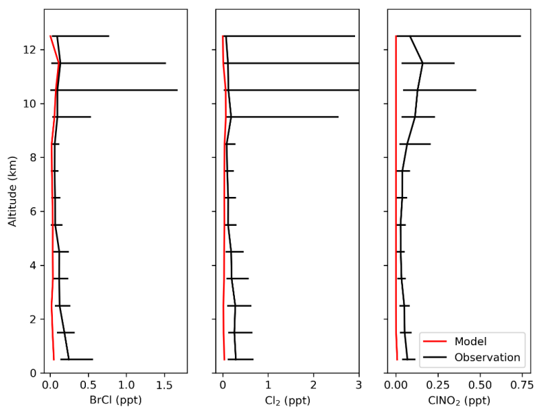
Figure 9b. Same as Figure 9a but for the ATom-4 campaign in April-May 2018.
