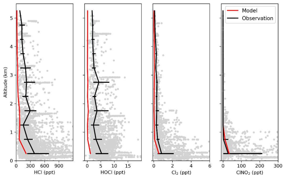
775 Figure 8. Vertical profiles of HCl, HOCl, Cl 2 , and nighttime CINO 2 mixing ratios during the WINTER campaign over the eastern US and offshore in February–March 2015. Observations are shown as individual 1 min data points, with medians and 25th–75th percentiles in 500m vertical bins. CINO 2 data exclude daytime (10:00–16:00 local) when mixing ratios are near zero in both the observations and the model. Model values are shown as medians sampled along the flight tracks.
