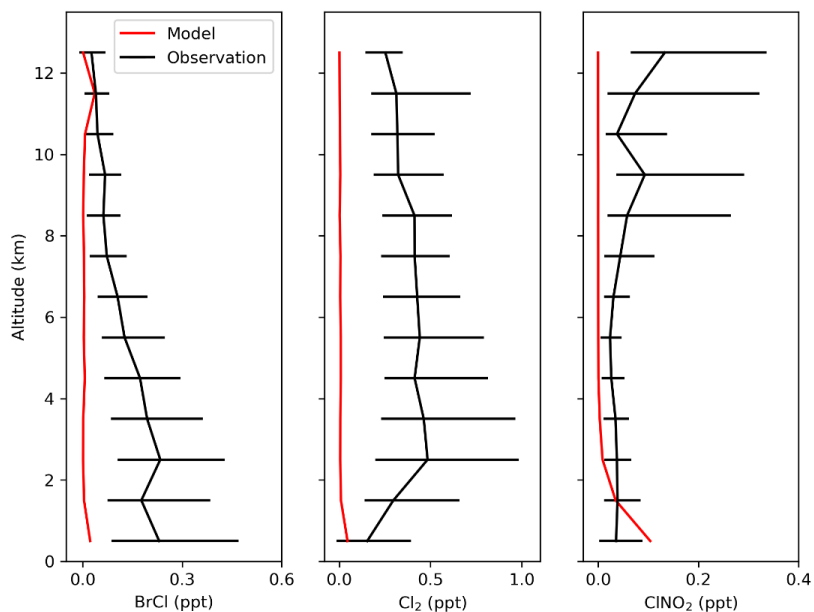
780 Figure 9a. Vertical profiles of BrCl, Cl 2 , and ClNO 2 mixing ratios from the ATom-3 campaign over the Pacific and Atlantic in September-October 2017. Observations are medians and 25th–75th percentiles in 1km vertical bins. Model values are medians sampled along the flight tracks.
