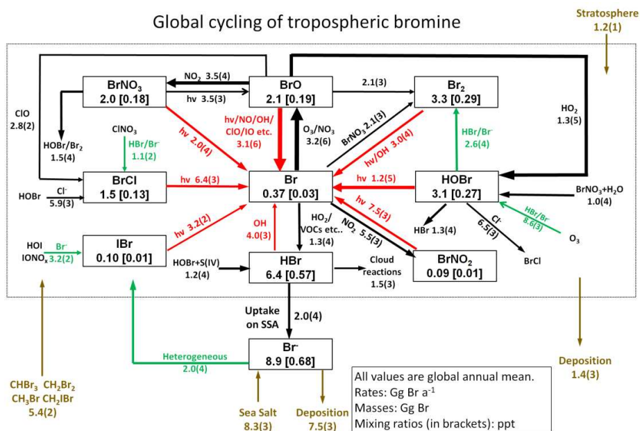
Figure 1b. Same as Figure 1a but for tropospheric inorganic bromine (Br y ).
