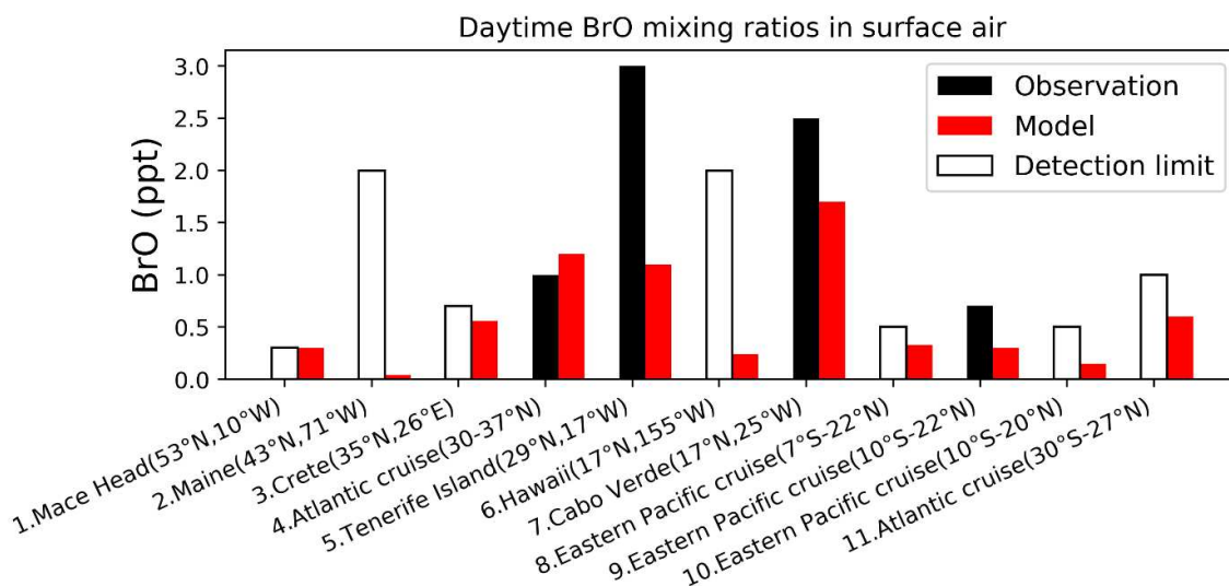
740 Figure 4. Daytime surface air mixing ratios of BrO from island sites and ocean cruises, arranged from left to right in order of decreasing latitude. Observed values (black) are means for the reporting period in different years. Open bars show the measurement detection limit and indicate that the observation is below detection limit. Model values (red) are monthly mean values in 2016 taken for the same month and location as the observations. References: (1) Saiz-Lopez et al., 2004; Saiz-Lopez et al., 2006; (2) Keene et al., 2007; (3, 5, 6) Sander et al., 2003; (4, 11) Leser et al., 2003; Martin et al., 2009; (7) Read et al., 2008; Mahajan et al., 2010; (8, 9) Volkamer et al. (2010); (10) 745 Volkamer et al. (2015).
