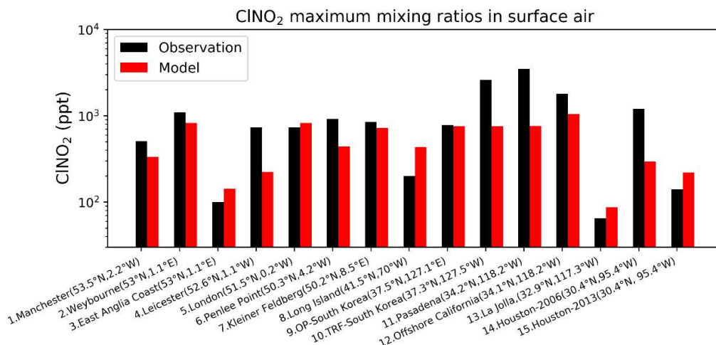
765 Figure 7. Surface air mixing ratios of CINO 2 at coastal and island sites, arranged from left to right in order of decreasing latitude. Observed (black) and modeled (red) values are maxima for the reporting period. Model maxima are based on hourly values sampled at the same location and time period as the observations. References: (1) Priestley et al. (2018); (2,4,6) Sommariva et al. (2018); (3,5) Bannan et al. (2017); (7) Phillips et al. (2012); (58) Kercher et al. (2009); (9,10) Jeong et al. (2018); (11) Mielke et al. (2013); (12) Riedel et al. (2013); (13) Kim et al. (2014) (14) Osthoff et al. (2008) (15) Faxon et al. (2015).
