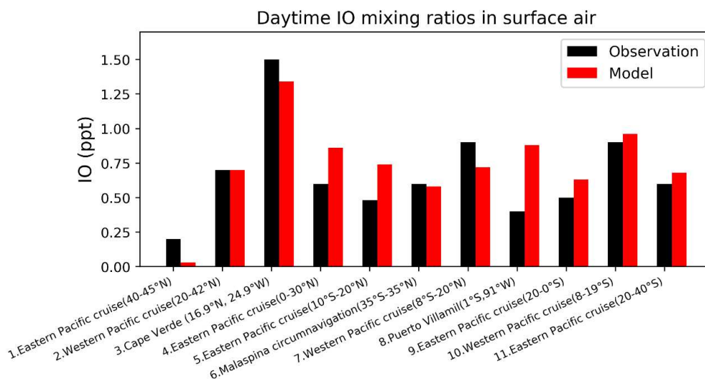
790 Figure 10. Daytime surface air mixing ratios of IO from island sites and ocean cruises, arranged from left to right in order of decreasing latitude. Observed values (black) are means for the reporting period in different years. Model values (red) are monthly mean values in 2016 taken for the same month and location as the observations. References: (1,4,9,12) Mahajan et al. (2012); (2,7,10) Großmann et al. (2013); (3) Mahajan et al. (2010); (5) Volkamer et al. (2015); (6) Prados-Roman et al. (2015); (8) Gómez Martín et al. (2013).
