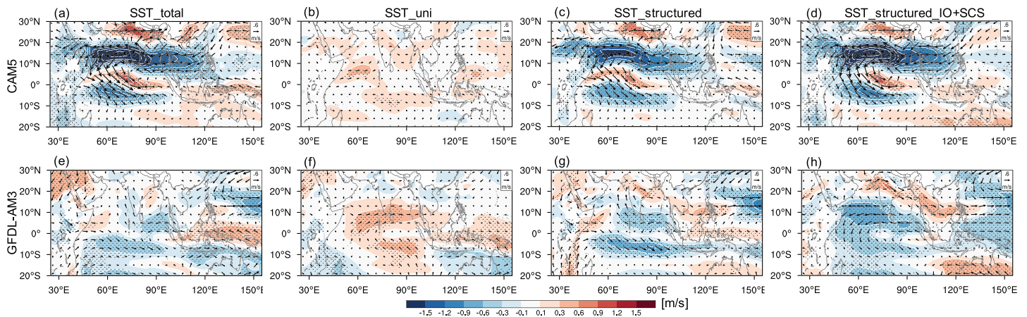
Figure 4. AGCM's 850 hPa wind response in the various SST experiments for CAM5 (top) and GFDL-AM3 (bottom). (a, e) Total aerosol-forced SST, (b, f) uniform cooling part of the SST, (c, g) spatially nonuniform but global SST pattern, and (d, h) nonuniform SST pattern over the Indian Ocean plus South and East China Seas. Stippling indicates statistical significance at the 5% level using a two-tailed Student's t test. Arrows show anomalous wind vectors and color shadings show anomalous wind speed in m/s.
