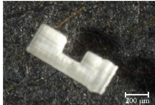
Figure 17. A micro-beam fabricated with DLP using clear IP-S resin photopolymer, where the smallest non-support feature is 86.7 \mu\text{m} . Twenty supports with a diameter of 3 \mu\text{m} were used during the building process. Here, the scale bar is 200 \mu\text{m} [114].
