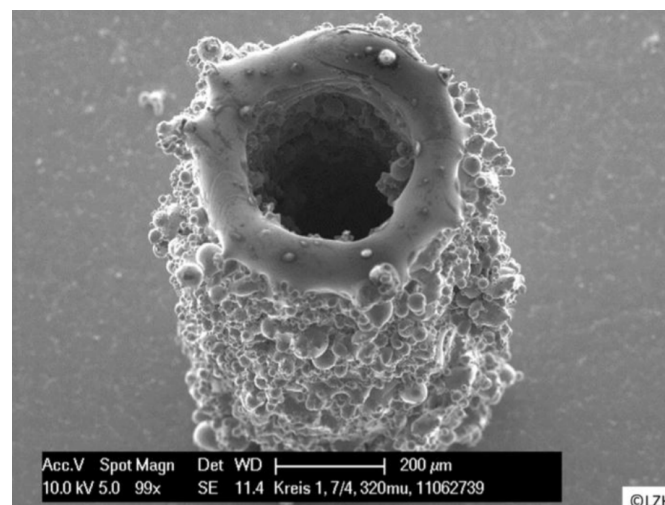
Figure 28. An SLM-fabricated micro-needle for drug delivery applications, where the needle was constructed from 316L stainless steel powder, with a length of 550 \mu\text{m} and an interior aperture measuring 160 \mu\text{m} across [145].
