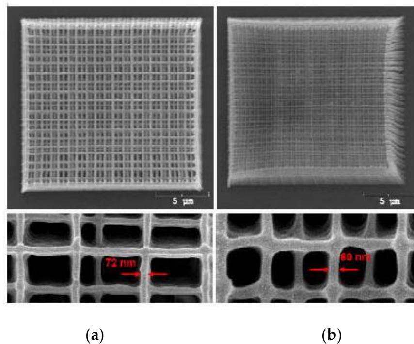
Figure 23. Nanoscale woodpile structures printed with MPP showing (a) laser excitation of 0.6 \mu\text{W} and a resultant beam thickness of 72 nm, and (b) laser excitation of 0.45 \mu\text{W} and a resultant beam thickness of 60 nm [126].
