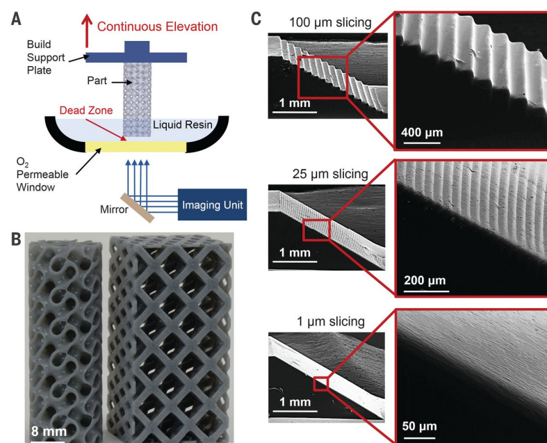
Figure 18. Gyroid structure printed in microscale with DLP showing (A) a diagram of the DLP set-up; (B) the gyroid part, printed at 500 mm/h; and (C) ramp test prints with slice thicknesses of 100 \mu\text{m} , 25 \mu\text{m} and 1 \mu\text{m} , successively. (From [115], Reprinted with permission from AAAS).
