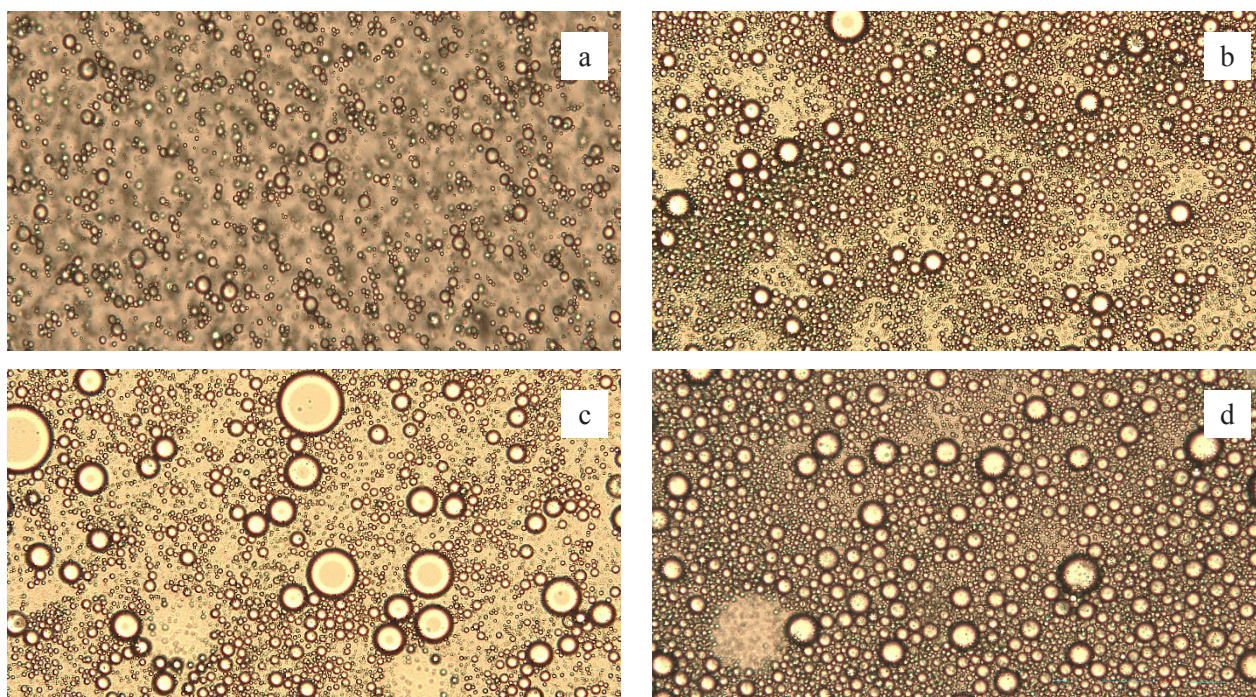
FIGURE 3. Optical microscope images of emulsion at 20×100 magnification, (a) Tween 20, (b) CMC, (c) WP, (d) WP/MD
