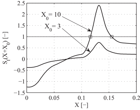
Fig. 9 Variation of S_f(X+X_0) as function of X . X_0 = 3 represents an example that fulfils the necessary condition for stability, while X_0 = 10 the equilibrium is unstable between 0.1162 < X < 0.155 .
