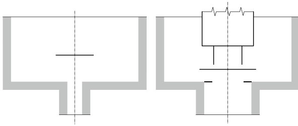
Fig. 1 Sketch of the poppet valves under analysis.
