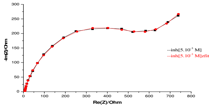
Figure 3: Nyquist curves for interface copper after treatment by 5.10^{-3} M C12N in a solution of 3% NaCl (--) experimental curve; (--) Curve fitted.
