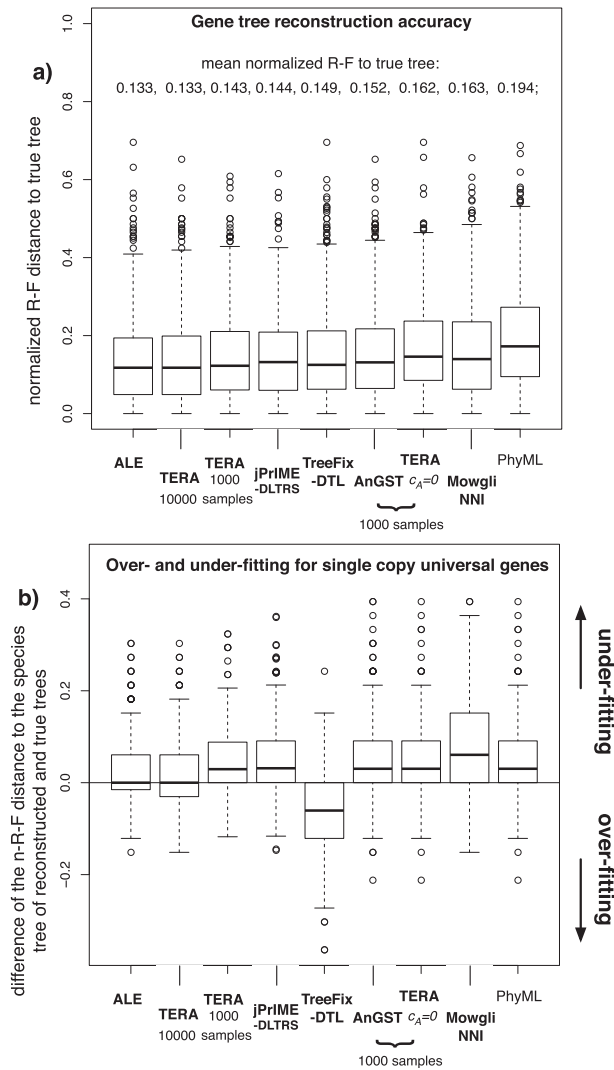
Fig. 2. (a) To compare the accuracy of TERA and other methods we used the simulated data set of Szöllősi et al. (2013b). We find that TERA achieves statistically equivalent accuracy to ALE and better accuracy than the other methods, see main text for details. (b) To test for over and underfitting of the species tree we examined the 431 gene families with exactly one copy in each of the 36 cyanobacterial species. For each family we plot the difference of the R-F distance of the true tree to the species tree and the R-F distance of the reconstructed gene tree from the species tree. Negative values for the difference indicate overfitting, while in the case of underfitting we expect a positive value
